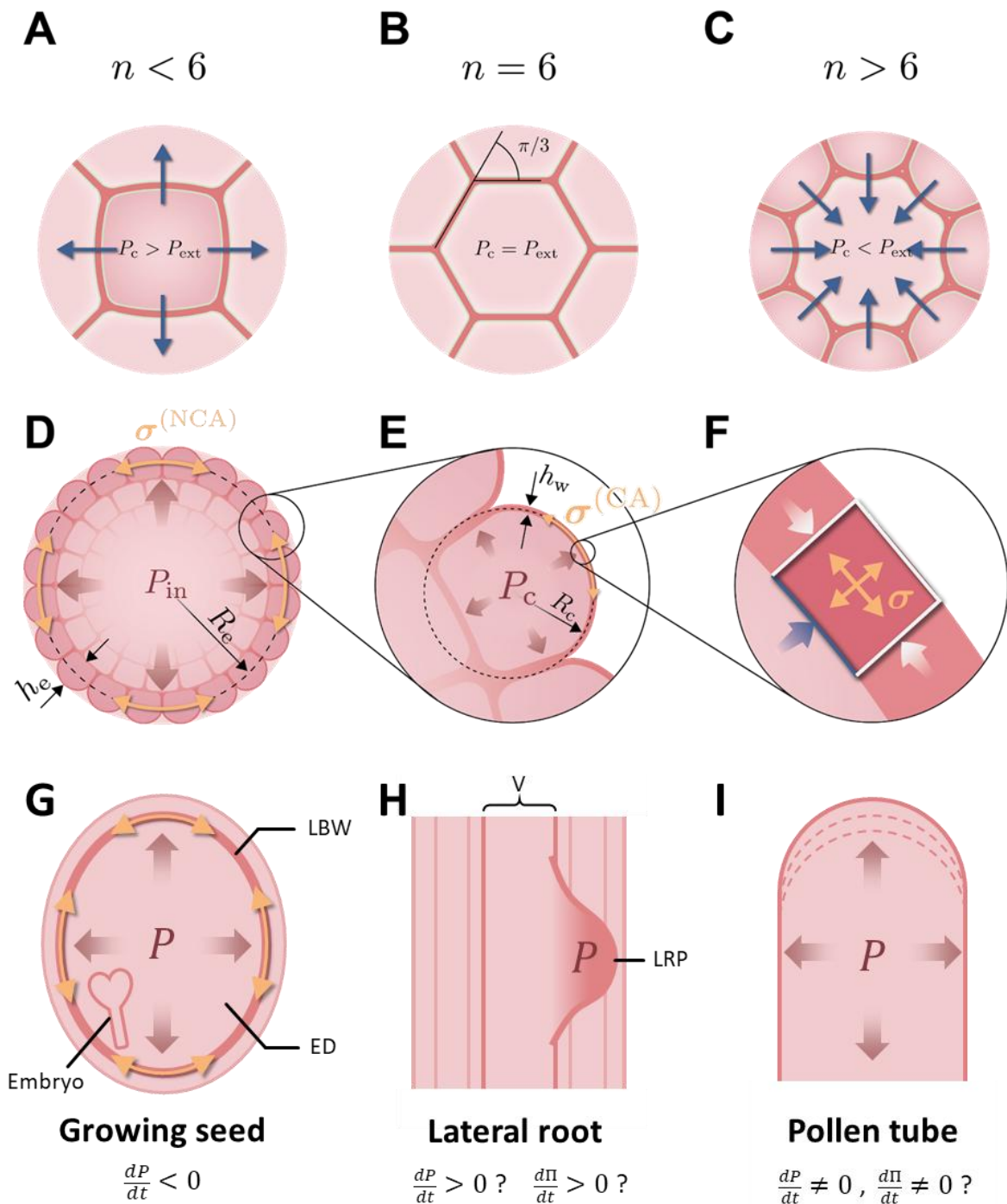
Figure 2. A, B, C: Qualitative relation between topology (number of neighbors n ), cell inner pressure ( P_c ) compared to the pressure of neighboring cells ( P_{ext} ), and water fluxes (blue arrows). By analogy with foam, cells with less than six neighbors feature higher pressure than their surroundings and tend to exhibit convex walls. Adapted from (Cantat et al. , 2013). D, E, F: Effect of turgor pressure across scales. (D) At the organ
