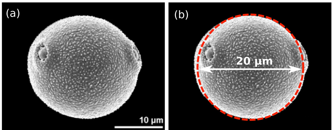
Figure 1. Pollen grain microscopy. (a) Birch ( Betula pendula ) pollen grain (source: Halbritter et al. 10 ); (b) showing an approximated spherical shell of 20 µm diameter (red color dashed-curve) used in the present computational model.
