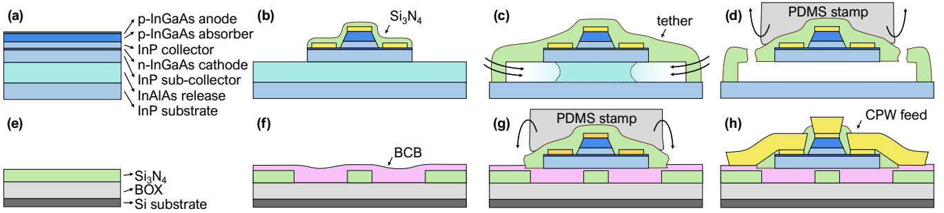
FIG. 2: Fabrication flow (a) Epitaxial growth of the source III–V wafer (b) Creating a diode by etching the mesa, depositing anode and cathode contacts, and SiN passivation. (c) After tethering the diode to the substrate with a new layer of SiN, the release layer is etched away. (d) This suspended coupon is then picked up by a PDMS stamp of the micro-transfer-printer. (e) The silicon target wafer with 300 nm SiN on top of the BOX. (f) Waveguides are created and a thin layer of BCB is spin-coated. (g) The coupon is then printed on top of the waveguide and (h) post-processed to create electrical contacts.
