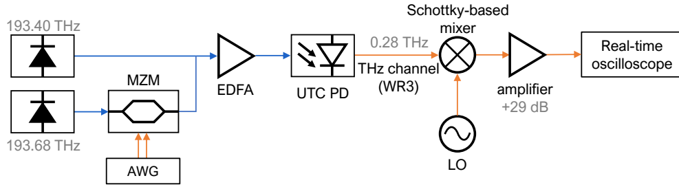
FIG. 3: In the experimental setup, two separate lasers are used for photomixing. One line is modulated using a MZM, before being combined and amplified by an EDFA. The light is coupled into the PIC using a vertical grating coupler and the mixed terahertz signal is then transferred over a WR3 waveguide channel before down-mixing, post-amplification, and sampling.
