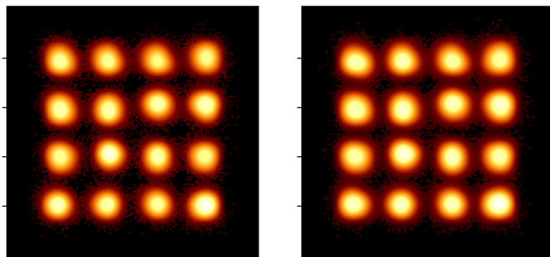
(a) 16-QAM at 35 GBd ( -1 V) with an EVM of 11.2 %.
