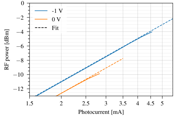
FIG. 5: RF power at 100 GHz. The 1 dB-saturation current for a PD with a 2 \times 16 \mu\text{m}^2 active area is above 4.6 mA for -1 V bias and 2.8 mA at zero bias.
