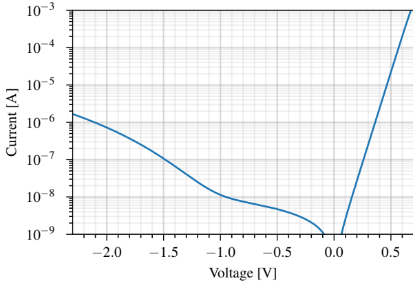
FIG. 4: The dark current for a PD with a 2 \times 16 \mu\text{m}^2 active area is below 10 nA for a bias voltage above -1 V.
