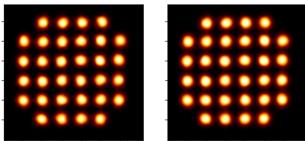
(c) 32-QAM at 25 GBd ( -1 V) with an EVM of 7.0 %.
