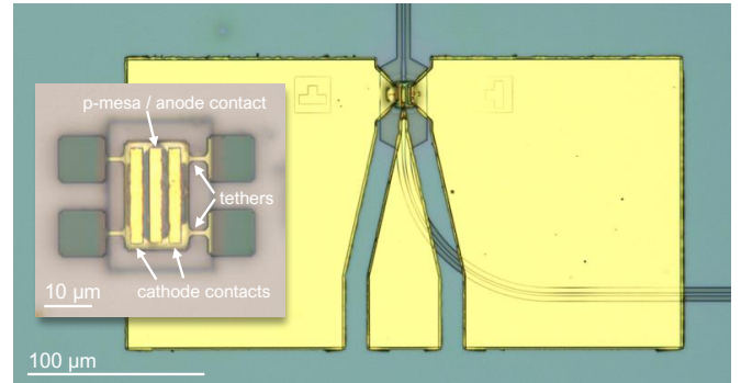
FIG. 1: A UTC PD is integrated on a SiN platform by transfer-printing a coupon (inset) on a waveguide.
