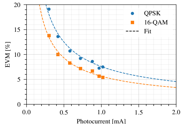
FIG. 8: The EVM for a 4 GBd transmission shows a clear inversely-quadratic fit with no deterioration for increased photocurrents.
