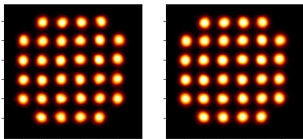
(c) 32-QAM at 25 GBd ( -1 V) with an EVM of 7.0 %.
