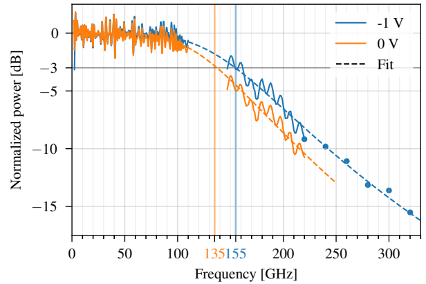
FIG. 6: The 3-dB bandwidth for a PD with a 2 \times 12 \mu\text{m}^2 active area is 155 GHz at -1 V bias and 135 GHz at zero bias, both with a photocurrent of 1 mA.
