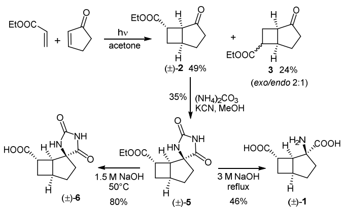
Scheme 1. Synthesis of ( ± )- 1 .
