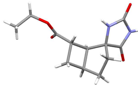
Figure 2. X-ray structure of compound ( ± - 5 ).
