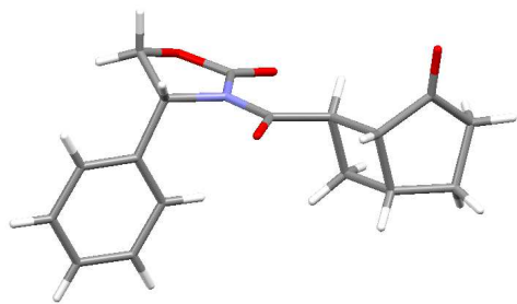
Figure 3. X-ray structure of compound 7b .
