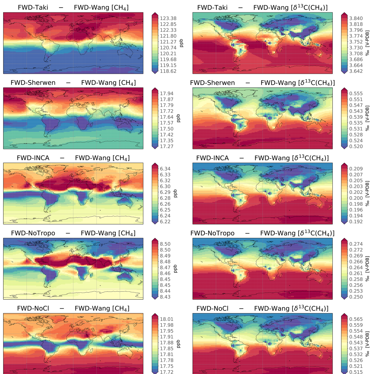
Figure 2. Surface absolute bias between FWD-* and FWD-Wang simulations averaged over 2010–2018. Temporal averaging is performed before subtraction. The left column displays the biases between the CH 4 mole fractions. The right column shows the biases between the δ 13 C(CH 4 ) values. Note that the scales are different for each panel.
