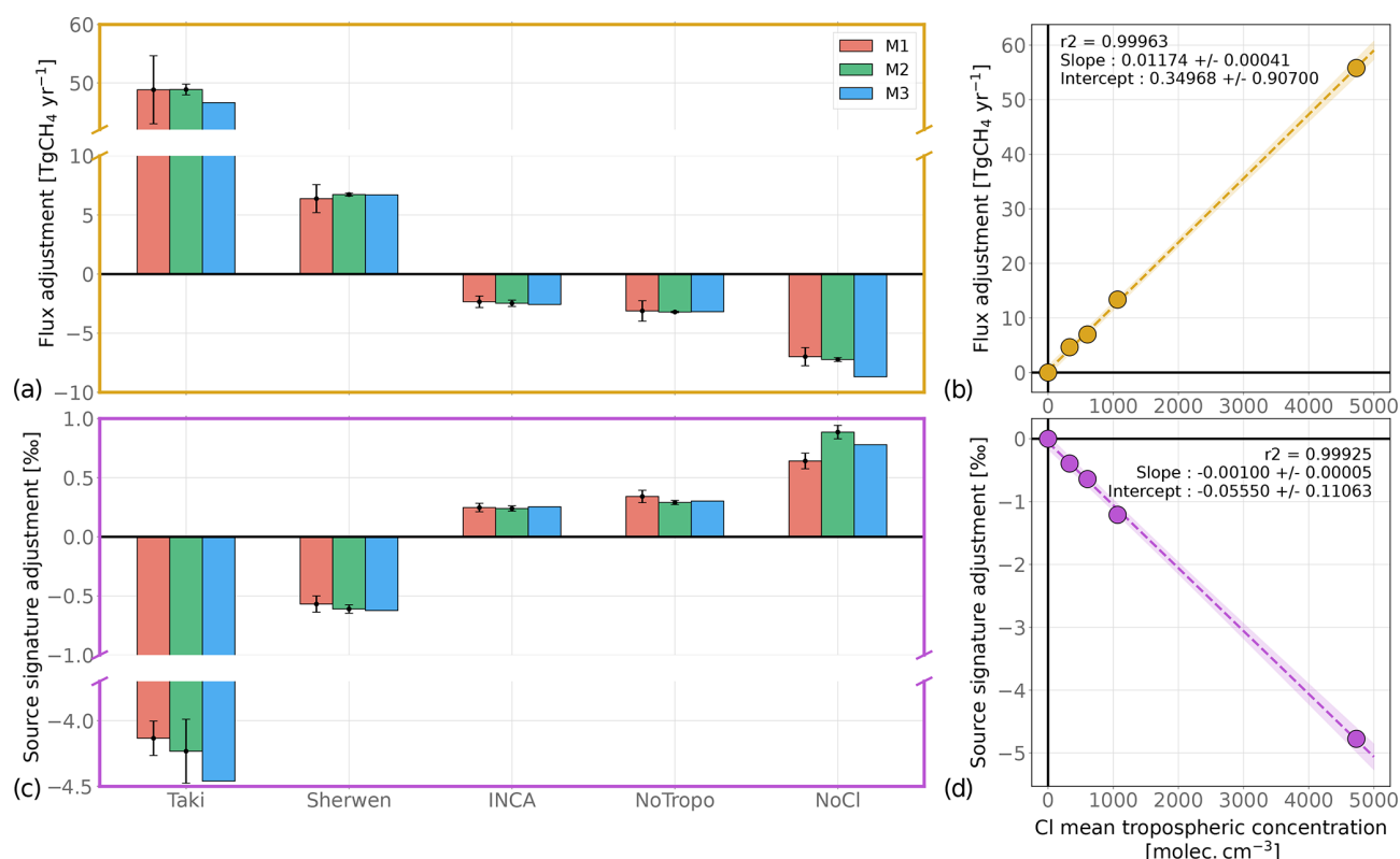
Figure 3. Global CH 4 flux and δ 13 C(CH 4 ) source source signature adjustment due to a change in the prescribed Cl field. Panels (a) and (c) show the adjustments for the global CH 4 flux (a) and δ 13 C(CH 4 ) source source signature (c) with the multiple methods (M1, M2, and M3) presented in Sect. 2.5 and Sects. S1, S2 and S3. Simulations with Cl-Wang are taken as a reference. For M1 and M2, the error bars correspond to the interannual variations (1 standard deviation) of adjustments. Panels (b) and (d) display the linear model derived from the relationship between the adjustments (estimated with M1) and the mean tropospheric concentration of the prescribed Cl fields. For the linear regression only, simulations without the Cl sink (NoCl) are taken as a reference to calculate the adjustments.
