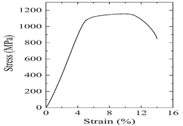
Figure 7. Stress-strain curve for 12% Cr ODS at RT (adopted from Shen et al. [69]).
