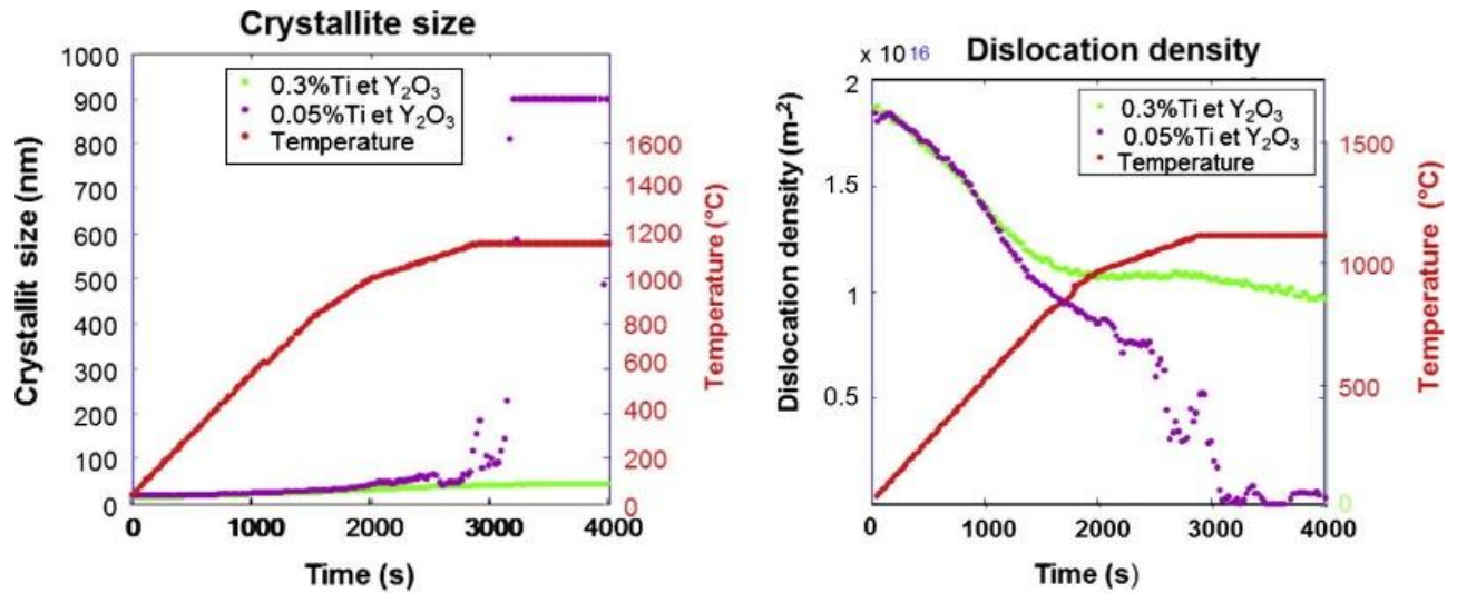
Figure 9. Variation in crystallite size and dislocation density as a function of time (adopted from Boutard et al. [73]).
