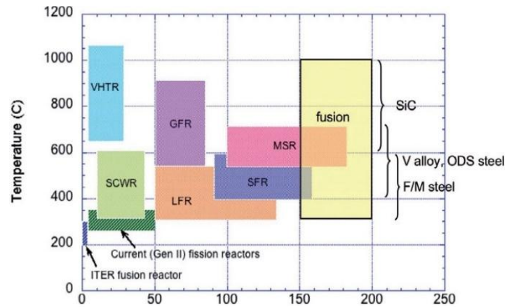
Figure 3. Relation of temperature and displacement per atoms (dpa) for GEN-IV reactors (adopted from Zinkle et al. [61]).
