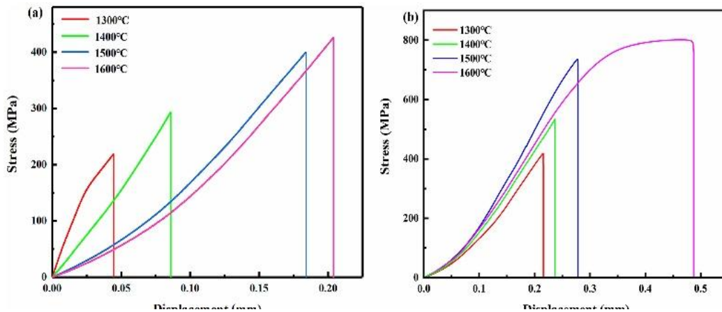
Figure 10. Stress-strain relation of ODS-tungsten at different temperatures (adopted from Liu et al. [74]).
