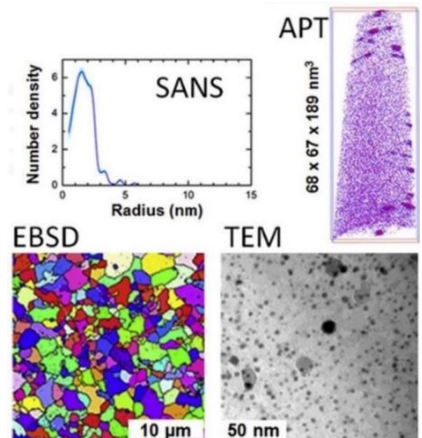
Figure 4. Microstructural characterization of strengthening in ODS (adopted from Chauhan et al. [66]).
