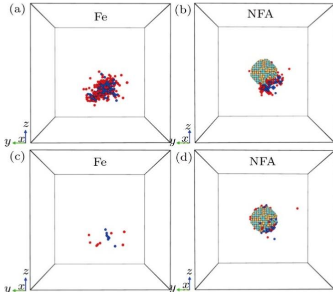
Figure 11. MD snapshot of displacement cascades observed for pure Fe and ODS at 20ps (adopted from Sun et al. [79]).
