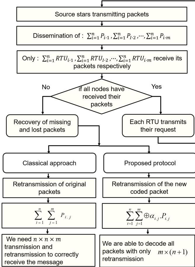
Fig. 3. Phases of operation of the proposed protocol.
