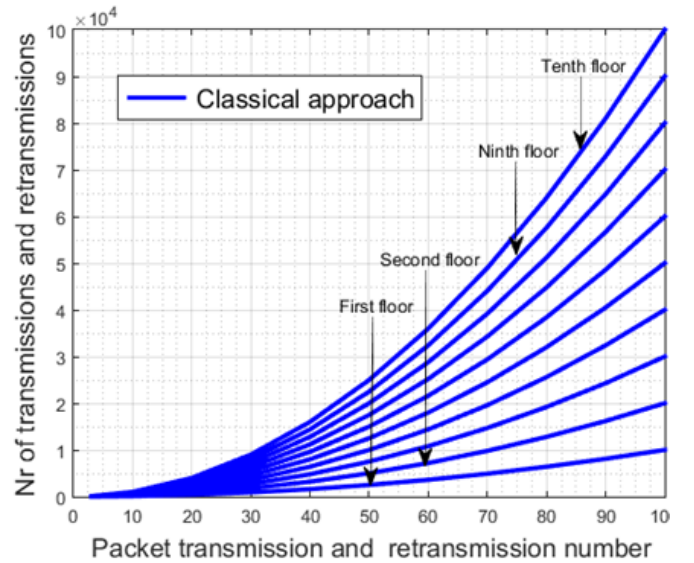
Fig. 4. Number of transmissions and retransmissions for the packets transmitted at different levels of the hospital by using the classical approach.
