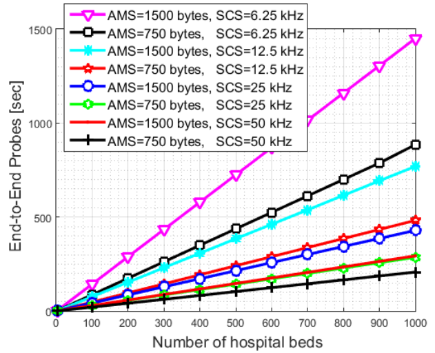
Fig. 7. PPerformance evaluation under different SCS values; N =3, and H = 1, AMS= 750/1500 bytes, and the QAM scheme is applied.
