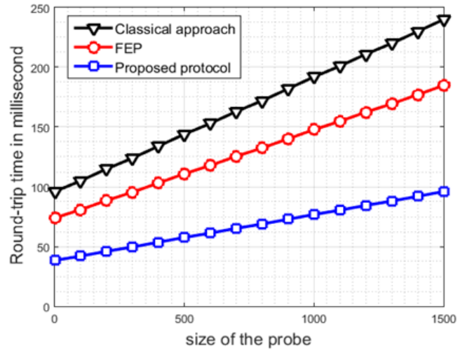
Fig. 13. RTT versus the probe size.
