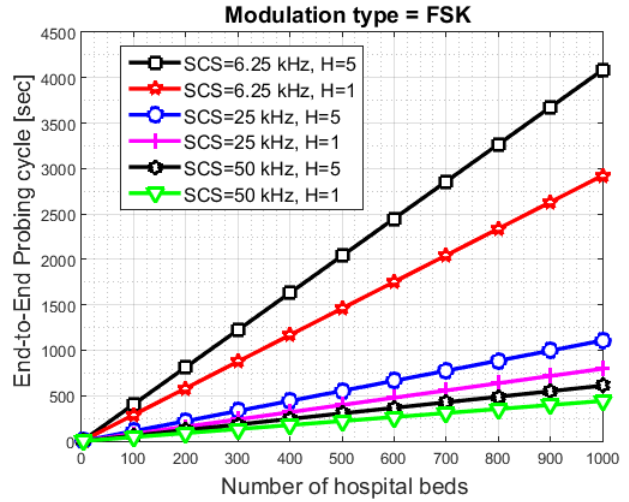
Fig. 10. E2E probing cycle versus the number of hospital beds for SCS 6.25 kHz, 25 kHz, and 50 kHz, using FSK.
