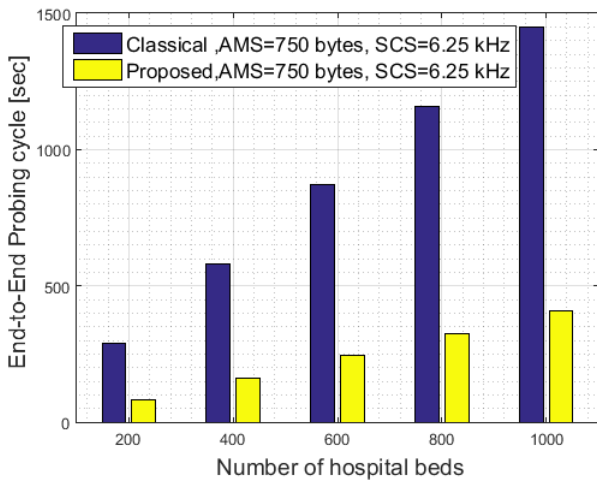
Fig. 12. Comparison between classical and proposed approaches.
