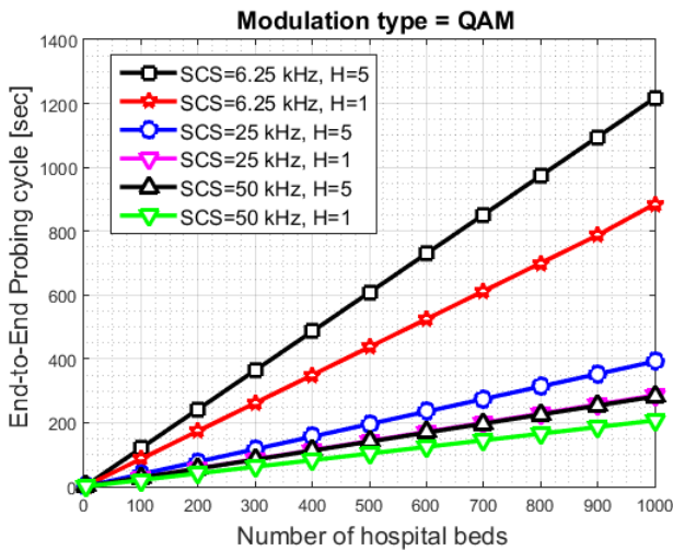
Fig. 9. E2E probing cycle versus the number of hospital beds for SCS 6.25 kHz, 25 kHz, and 50 kHz using QAM.
