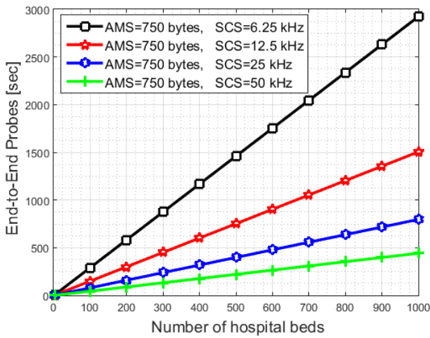
Fig. 8. Comparison and assessment of results under a subcarrier configuration of N = 50 , H = 1 with AMS = 750 bytes, using FSK.
