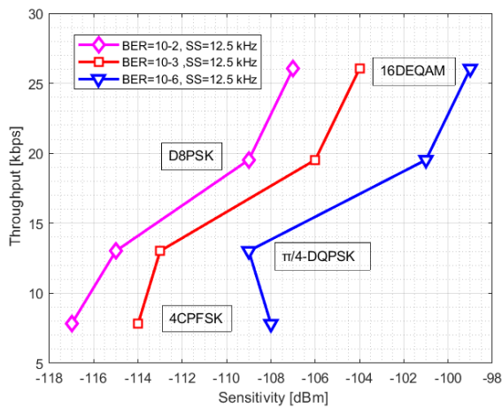
FIGURE 7. This figure shows the measurement results of throughput vs. maximum useable sensitivity for different linear and non-linear modulation techniques at SS = 12.5 \text{ kHz} : Conventional approach.
