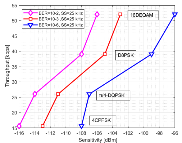
FIGURE 8. Conventional approach: Measurement results of throughput vs. maximum useable sensitivity for different linear and non-linear modulation techniques at SS=25 \text{ kHz} .
