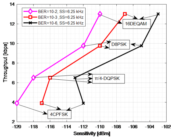
FIGURE 6. Conventional approach: Measurement results of throughput vs. maximum useable sensitivity for different linear and non-linear modulation techniques at SS = 6.25 \text{ kHz} .
