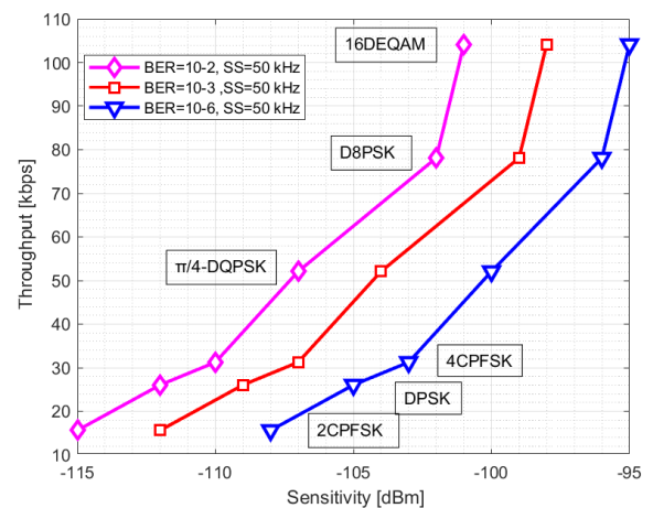
FIGURE 9. Conventional approach: Measurement results of throughput vs. maximum useable sensitivity for different linear and non-linear modulation techniques at SS=50 \text{ kHz} .
