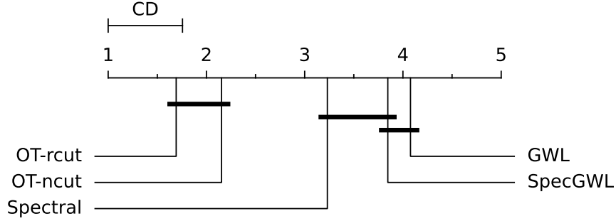
Figure 3: Neményi post-hoc rank test results. OT-rcut and OT-ncut outperform the comparative approaches in a statistically significant manner while having comparable performance.
