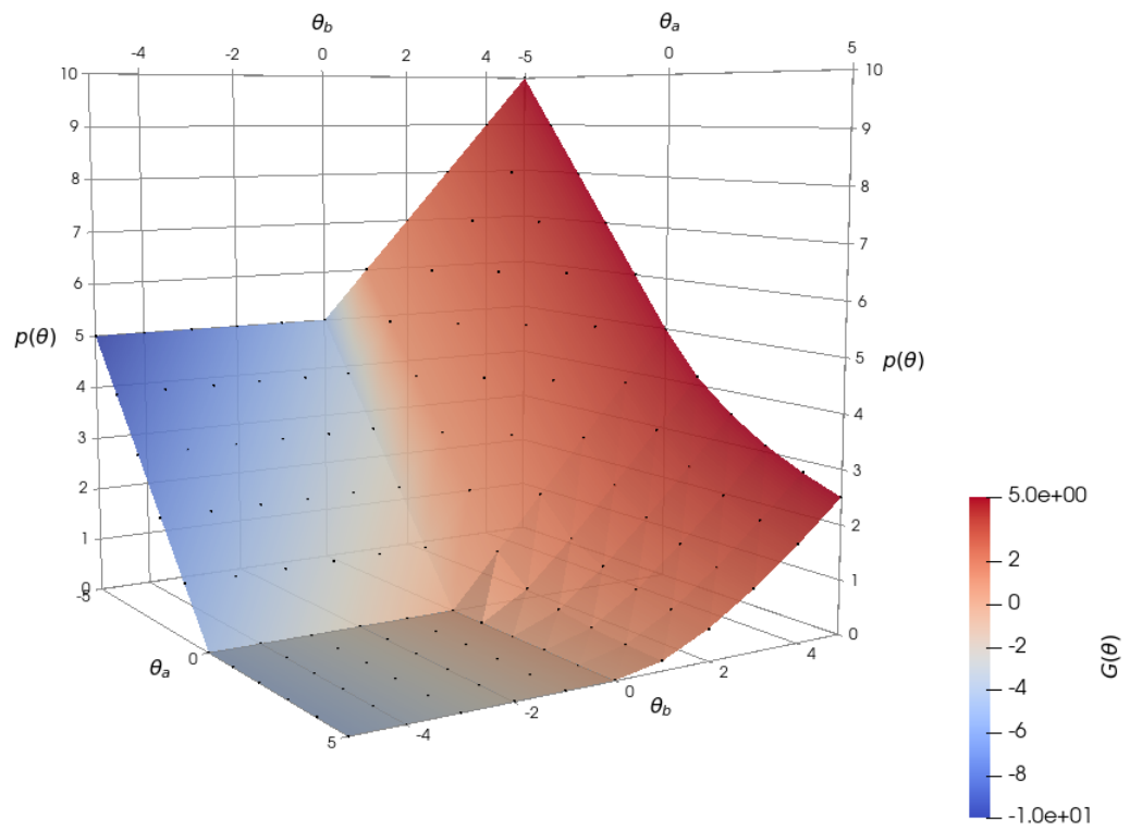
Figure 9: The price functional \theta \mapsto p(\theta) and the payoff mapping \theta \mapsto G(\theta)
