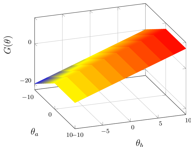
Figure 7: The payoff mapping \theta \mapsto G(\theta)
