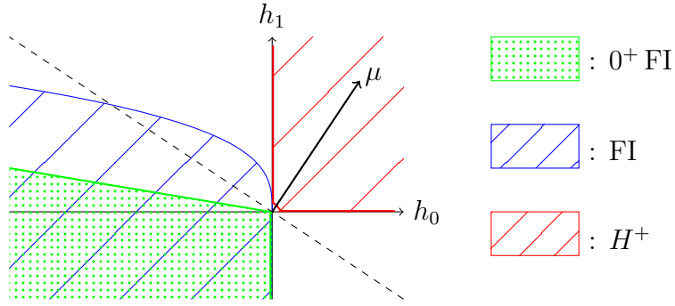
Figure 4: Geometry of no-arbitrage
