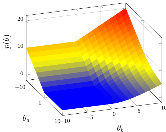
Figure 8: The price functional \theta \mapsto p(\theta)
