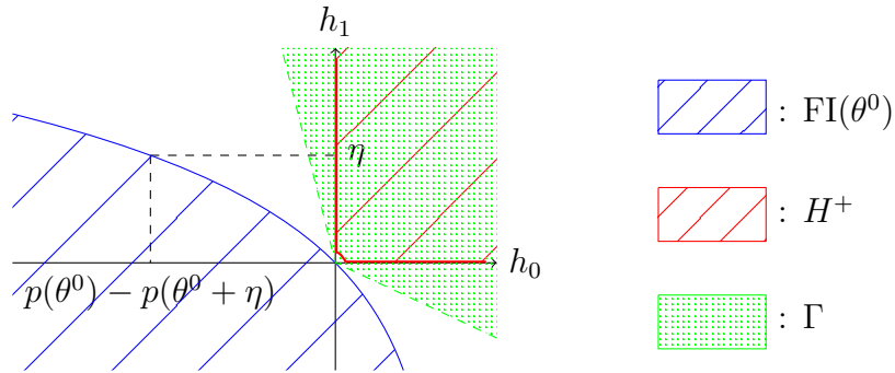
Figure 2: Geometry of robust no-arbitrage
