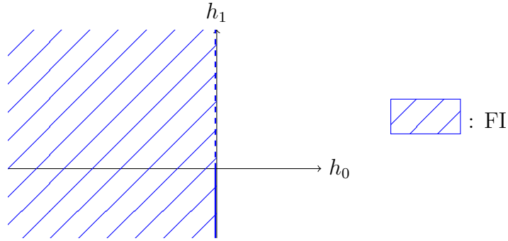
Figure 10: The set of financially feasible consumption increments is not closed.
