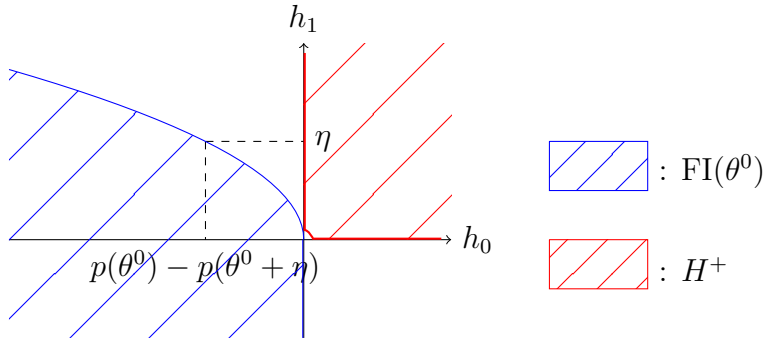
Figure 3: Geometry of no-arbitrage
