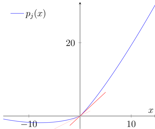
Figure 1: Price functional with market impact where \bar{p}_j^u = 1.3 , \underline{p}_j^u = 0.7 , \beta_j = 1/5 , and \gamma_j = 1/6 .
