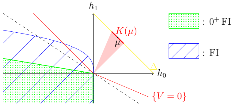
Figure 6: Indifference curve of V
