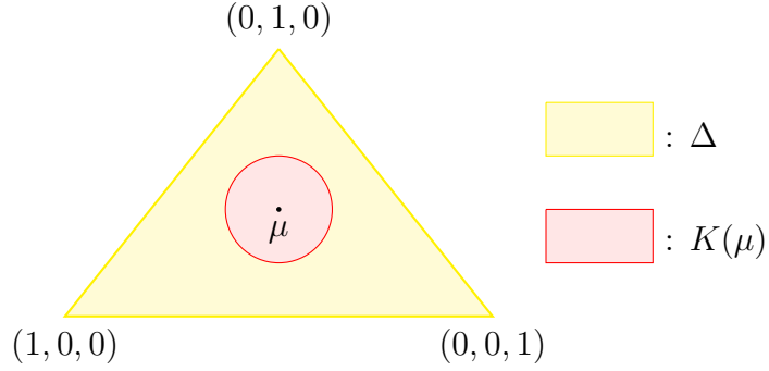
Figure 5: The set K(\mu) with two states of nature.
