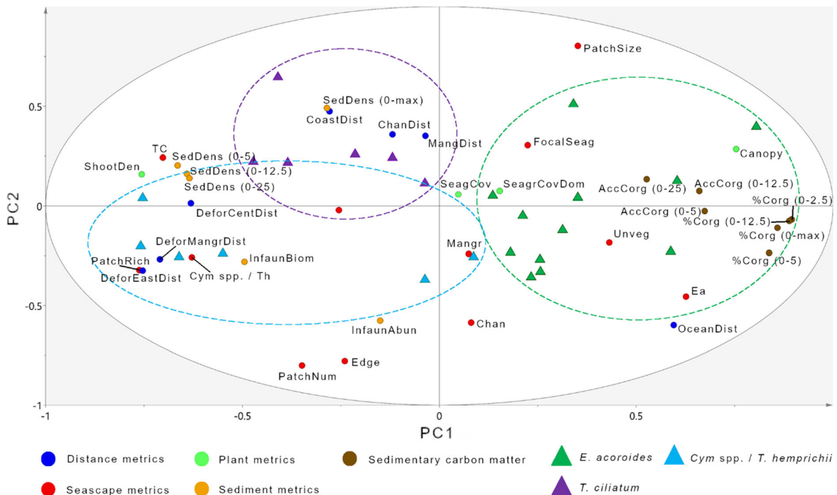
Fig. 4 Principal component analysis (PCA) biplot displaying correlative assessments of scale-dependent predictors (distance-, seascapes-, plant- and sediment-metrics), sedimentary C_{org} content at different depth sections and the model observation metrics of each seagrass seascape represented by Enhalus
