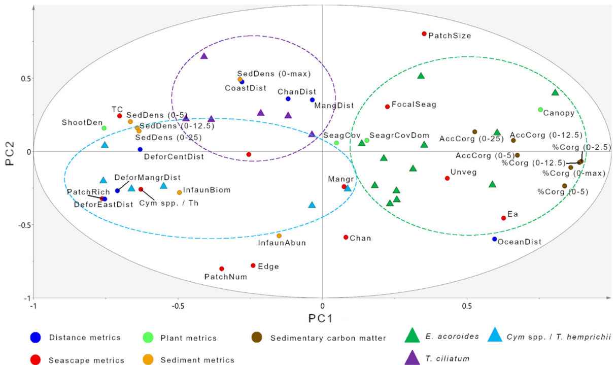
Fig. 4 Principal component analysis (PCA) biplot displaying correlative assessments of scale-dependent predictors (distance-, seascape-, plant- and sediment-metrics), sedimentary C org content at different depth sections and the model observation metrics of each seagrass seascape represented by Enhalus
