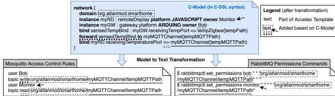
Fig. 5. Generation of Access Control Rules for Mosquitto and RabbitMQ using M2TT; Same information indicated with same sign; For RabbitMQ syntax, first argument (“ ”) is for configure permission, second for write permission and third for read permission.
