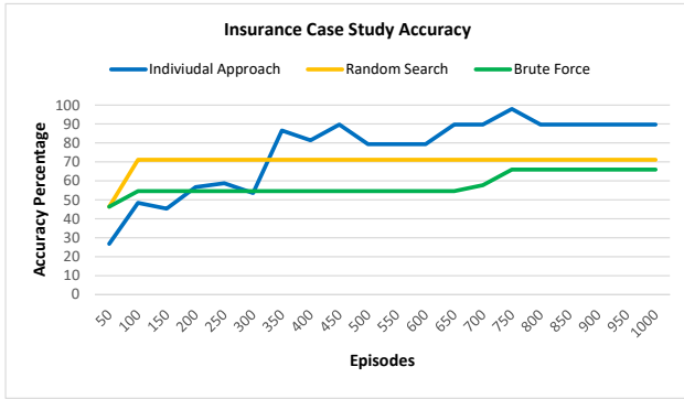
Fig. 12 The normalized accuracy of the individual approach in solving the Insurance case study
