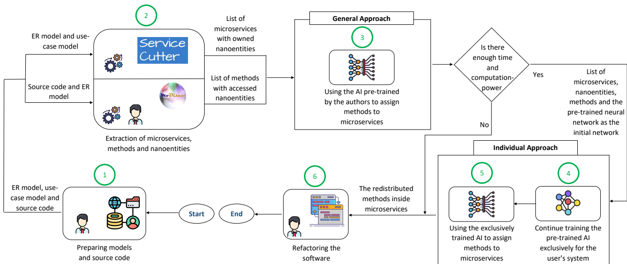
Fig. 5 The workflow of using the framework by the end-user consisting of six steps
