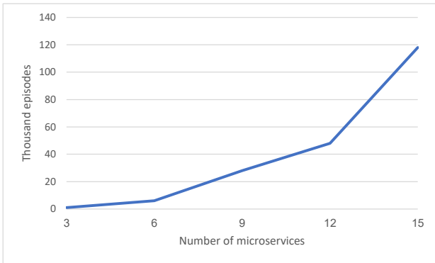
Fig. 15 Thousand episodes needed to reach 80% accuracy based on the maximum number of MSs in general approach
