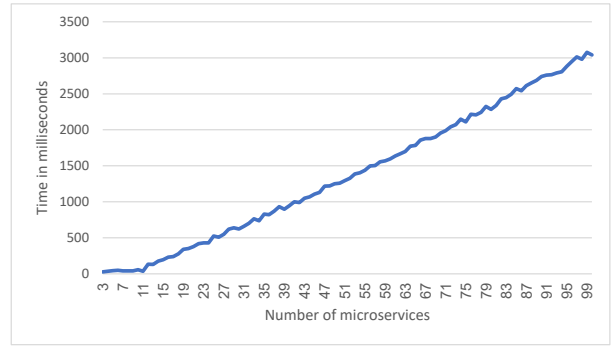
Fig. 14 Time needed for each episode of the training program to complete based on the number of MSs
