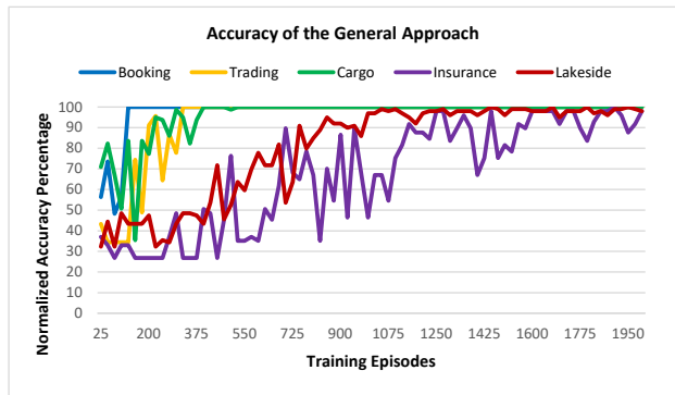
Fig. 8 The normalized accuracy of the general approach during training (graphical)
