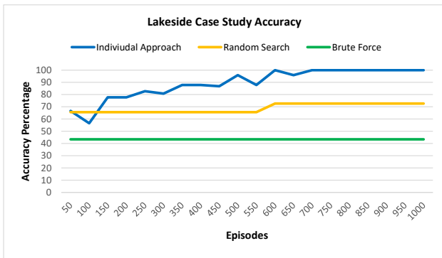
Fig. 13 The normalized accuracy of the individual approach in solving the Lakeside case study
