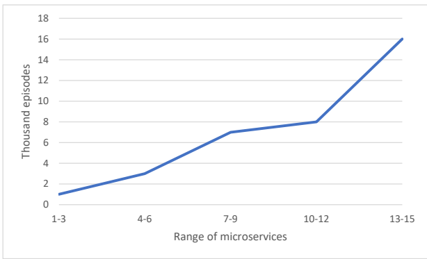
Fig. 16 Thousand episodes needed to reach 80% accuracy based on the range of MSs in the general approach
