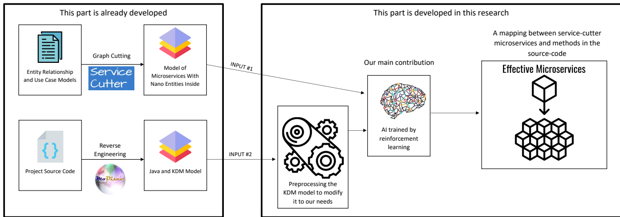
Fig. 4 The structure of the developed framework to facilitate migration to the MS architecture.
