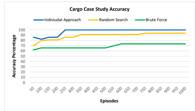
Fig. 10 The normalized accuracy of the individual approach in solving the Cargo Tracking case study
