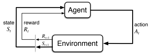
Fig. 3 The agent–environment interaction in a Deep Q-Learning problem [28]
