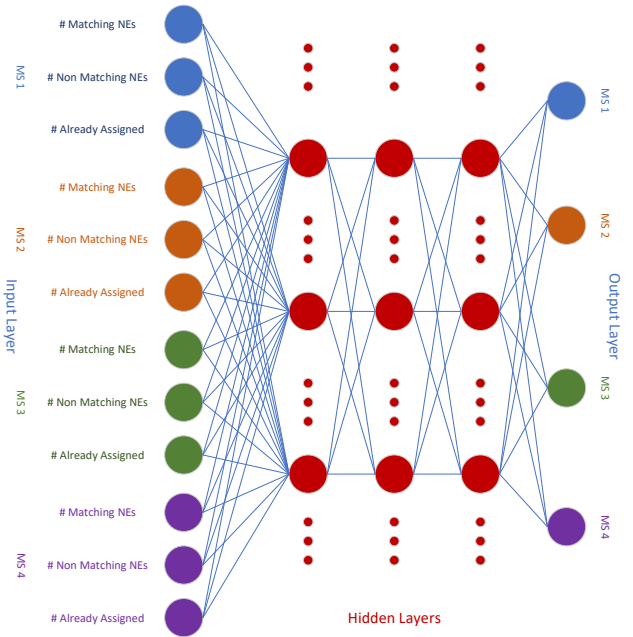
Fig. 6 The structure of the neural network used in the individual and the general approach
