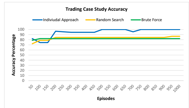
Fig. 11 The normalized accuracy of the individual approach in solving the Trading case study
