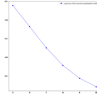
Figure 12: Log-error of the recursive quantization scheme (1.16)-(1.18)-(1.19) with respect to \log_2(K) . The slope is approximately equal to -0.436 .
