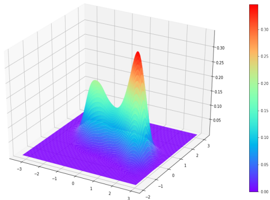
Figure 14: The simulated density function smoothed by the Gaussian kernel method (bandwidth = 0.241).
