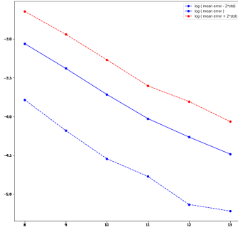
Figure 9: Log-error of the particle method (1.8) with respect to \log_2(N) . The slope is approximately equal to -0.285 .
