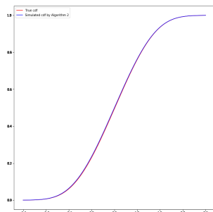
Figure 4: Simulation by the recursive quantization scheme with Lloyd's iteration (1.16)-(1.19)
