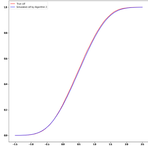
Figure 6: Simulation by the hybrid particle-quantization scheme without Lloyd iteration (1.22)
