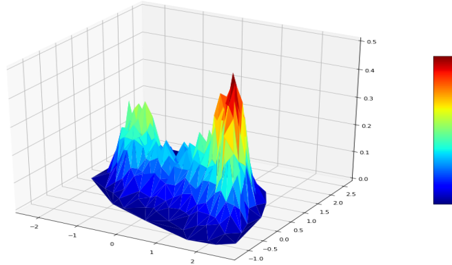
Figure 17: The density function simulated by the hybrid particle-quantization method (1.22). The vertical axis is the weight divided by the area of the corresponding Voronoi cell.
