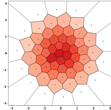
Figure 2: The quadratic optimal quantization for the standard normal distribution \mathcal{N}(0, \mathbf{I}_2) .
