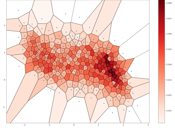
Figure 16: The Voronoi cells of the above quantizer. The colour of each Voronoi cell represents the weight of this cell (the darker the heavier).
