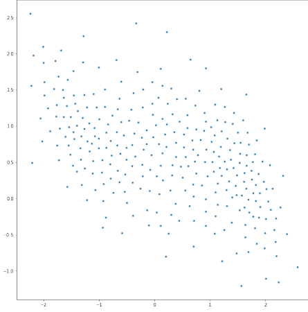
Figure 15: The quantizer of (x_0, x_1) , simulated with particle number N = 5000 , quantizer size K = 300 and 10 Lloyd iterations at each Euler step.
