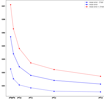
Figure 8: Error of the particle method (1.8) with respect to the particle size N
