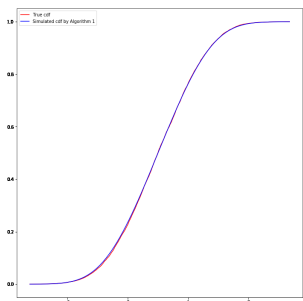
Figure 3: Simulation by the particle method (1.8)
