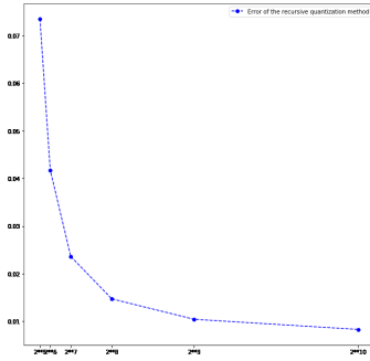
Figure 11: Error of the recursive quantization scheme (1.16)-(1.18)-(1.19) with respect to the quantizer size K
