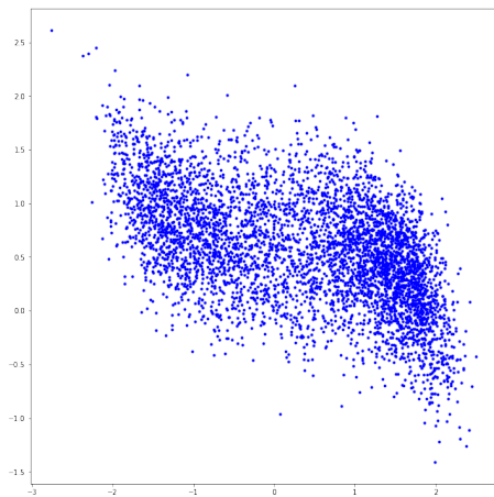
Figure 13: The first and second coordinates of 5000 particles at time T = 1.5 .
