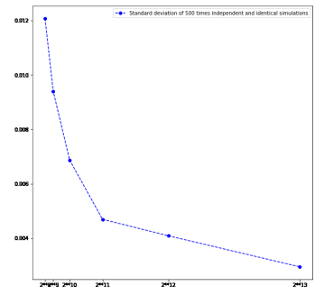
Figure 10: The standard deviation of the error of the particle method (1.8) with respect to N
