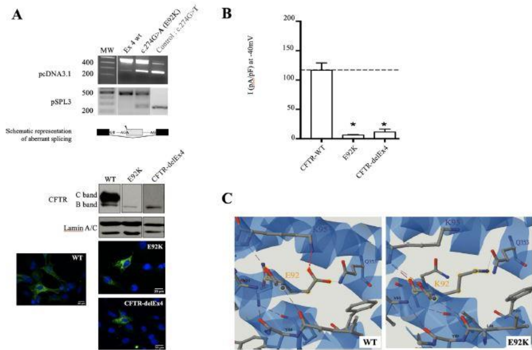
Fig. 3. Results of the functional experiments in BEAS-2B and/or HeLa cell lines for the variant c.274G > A (E92K).
