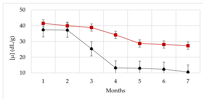
Figure 6. Intrinsic viscosity [\eta] as a function of time. Storage and tests performed at T = 60\text{ }^{\circ}\text{C} . Nanofluid (—■). Polymer solution (—●).
