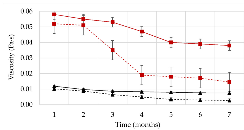
Figure 5. Viscosity as a function of time at a shear rate of 7.3 \text{ s}^{-1} . Storage and measurement at T = 60 \text{ }^{\circ}\text{C} . Semi-dilute nanofluid (1000 ppm XG, 300 ppm NP-SiO 2 and 3% NaCl) (—■). Semi-dilute polymer solution (1000 ppm XG and 3% NaCl) (---■). Dilute nanofluid (400 ppm XG, 300 ppm NP-SiO 2 and 3% NaCl) (—▲). Semi-dilute polymer solution (400 ppm XG and 3% NaCl) (---▲).
