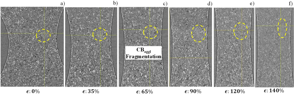
Figure A3: a)-f) evolution of CB aggl during a tensile test in material S_9.0 observed using SRCT. CB aggl are fractured between 35%-65%, to be precise at 40% nominal strain. CB aggl undergo multiple fragmentations as the macroscopic deformation increases.
