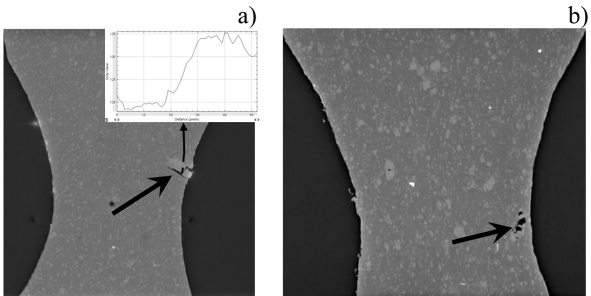
Figure A5: Slice images showing critical defects. The defects pointed in the images are \text{CB}_{\text{aggl}}
