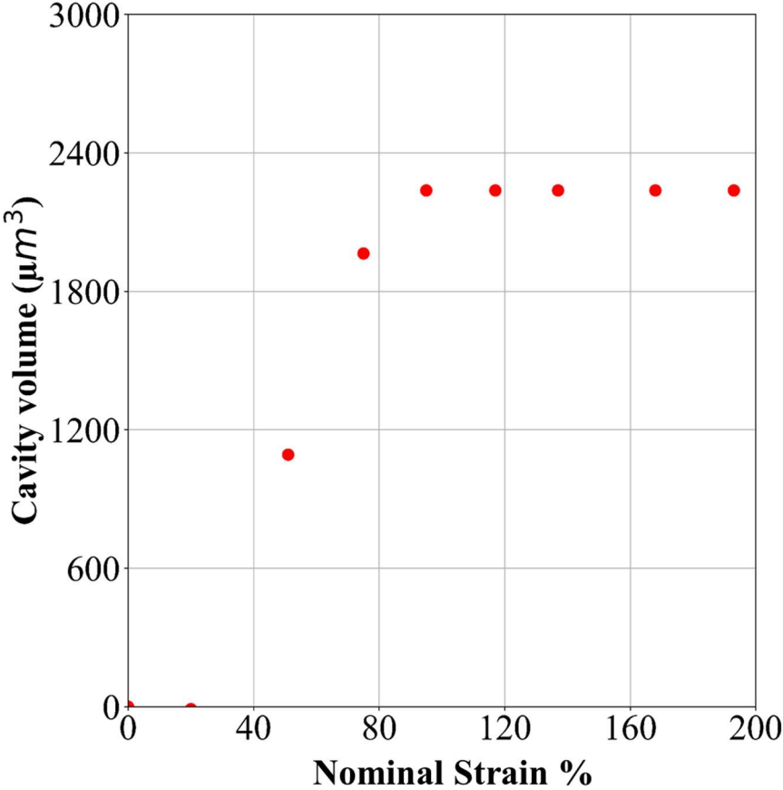
Figure A2: Evolution of cavity associated to a defect with E_{q_{diam}} = 23\mu m
