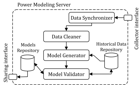
Figure 3: Power Modeling Server Architecture
