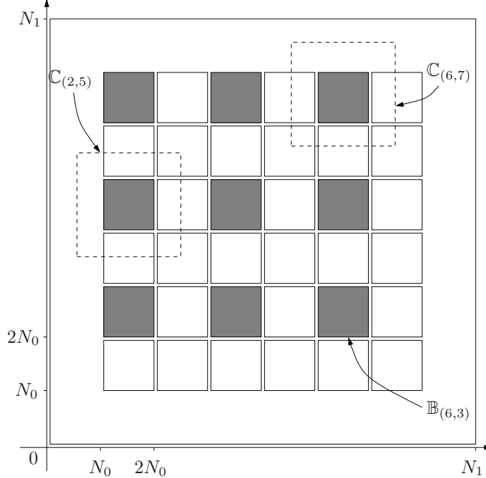
FIGURE 1. The set \tilde{\Lambda}_{N_1} is drawn for d = 2 (we need it only for d \geq 3 , but for illustration purposes d = 2 is enough) and N_1 = 8N_0 . The set \Lambda_{N_1, N_2}^- is the (disjoint union) of the B_j 's boxes, j \in \{2, 3, 4, 5, 6, 7\}^2 = \cup_{w \in \{0, 1\}^2} \mathcal{J}_w . We have singled out \Lambda_{N_1, N_0}^{(0,1)} by making it darker: observe that \Lambda_{N_1, N_0}^- is the disjoint union of \Lambda_{N_1, N_0}^w, w \in \{0, 1\}^2 . We have also drawn, with dashed boundaries, some of the \mathbb{C}_j boxes.
