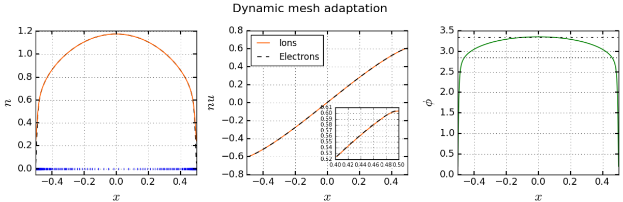
FIGURE 10. Number density, momentum and electric potential profiles at final time t_f = 4t_0 . Plasma parameters: \varepsilon = 1/1836 , \kappa = 0.0025 , \bar{\lambda}_D = 0.002 , no collision. Numerical scheme: Modified Lie splitting, controlled diffusion Rusanov solver for electron and scaled diffusion fixed HLL solver for ions. Simulation parameters: \Delta x ranges from 2^{-5} to 2^{-10} , \Delta t \approx 6 \times 10^{-6} . The vertical blue markers materialize the centers of the cells.
