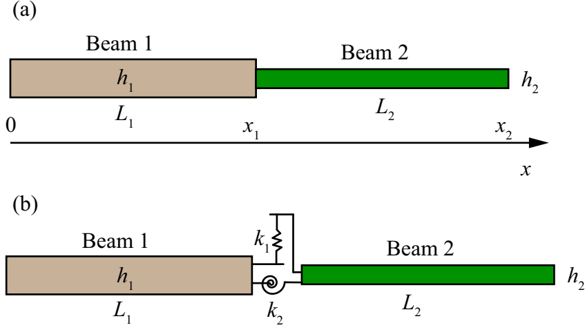
Figure 1: Illustration of (a) two fully coupled beams with different thickness, and (b) the two beam substructures connected by artificial springs, in which k_1 and k_2 respectively control the bending displacement and rotational angle differences at the joint. Artificial springs are only applied at the connected boundaries of each beam while global boundary conditions (zero external force and moment in this case) are imposed at the non-connected ends of the beams. Note also that the axial vibration is not considered and when k_1 \rightarrow +\infty and k_2 \rightarrow +\infty case (a) is recovered.
