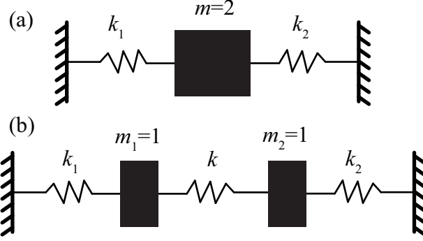
Figure A1: (a) Illustration of a resonator having two springs in parallel. (b) Illustration of dividing the resonator into two and assembling them by an artificial spring k .
