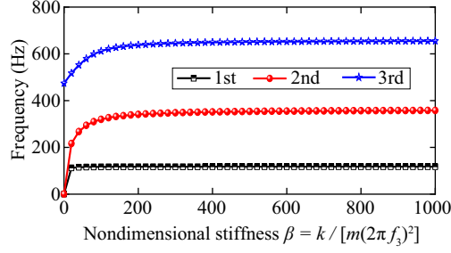
Figure 3: Influence of the artificial spring stiffness on the first three modal frequencies of the two-beam model, to see how convergence depends on the spring stiffness value. Here m = 1 stands for the normalized modal mass and f_3 for the 3-rd eigenfrequency of Beam 2.
