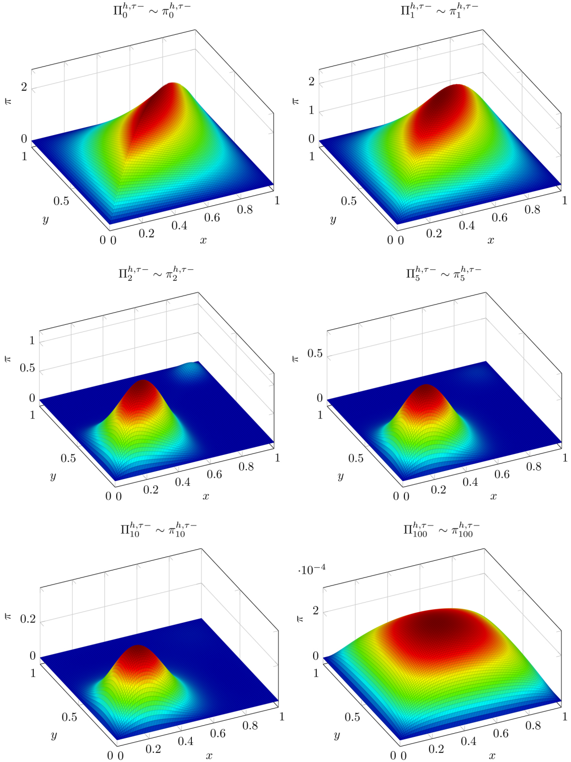
FIGURE 1. Kernel evolution \pi(x, x', t) at different time step t = 0, \tau, 2\tau, 5\tau, 10\tau, 100\tau , approximated with \pi_n^{h, \tau, -} \sim \Pi_n^{h, \tau, -} , with n \in \{0, 1, 2, 5, 10, 100\} .
