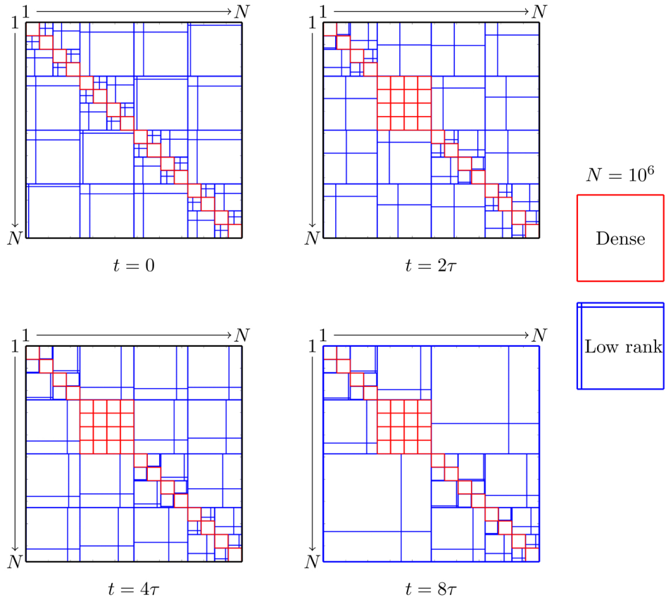
FIGURE 6. \mathcal{H} -matrix evolution for the advection-diffusion equation.
