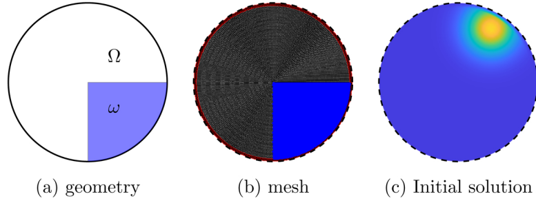
FIGURE 5. Geometry, mesh and initial condition of the advection-diffusion problem.
