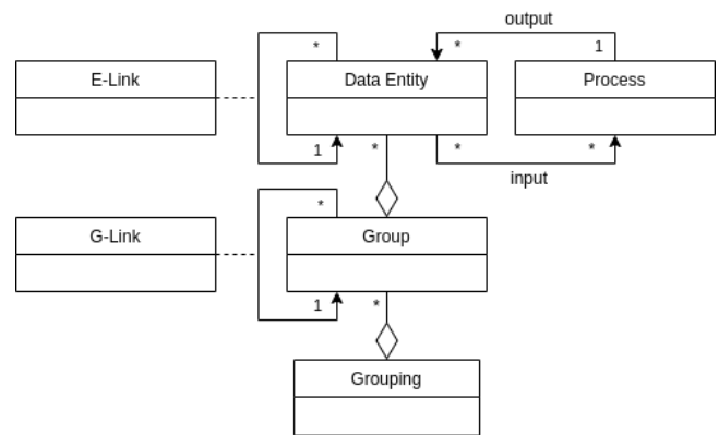
Figure 1: goldMEDAL concepts (UML class diagram)
