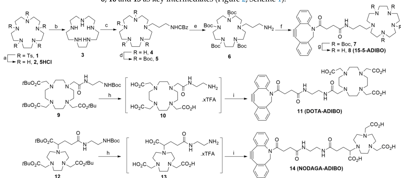
Scheme 1. Synthesis of 15-5 precursor 6 and 15-5-, DOTA- and NODAGA-ADIBO conjugates 8 , 11 and 14 : (a) (i) conc. \text{H}_2\text{SO}_4 , 110^\circ\text{C} , 48 h; (ii) conc. aq. \text{HCl} , RT, 15 h; (b) aq. \text{NaOH} , toluene, Dean-Stark, overnight; (c) benzyl 3-bromopropylcarbamate ( S11 ), \text{Et}_3\text{N} , \text{CHCl}_3 , RT, 34 h; (d) \text{Boc}_2\text{O} , \text{Et}_3\text{N} , \text{CHCl}_3 , RT, 18.5 h then 50^\circ\text{C} , 1 h; (e) \text{H}_2 , Pd/C 10%, i PrOH, RT, 48 h; (f) ADIBO-NHS S10 , DIPEA, \text{CH}_3\text{CN} , RT, 30 h; (g) TFA, anisole, \text{CH}_2\text{Cl}_2 , 0^\circ\text{C} , 2 h then RT, 1 h; (h) TFA, anisole, -10^\circ\text{C} then RT, 20–23 h; (i) ADIBO-NHS S10 , DIPEA, DMSO, RT, 2.5–3 h.
