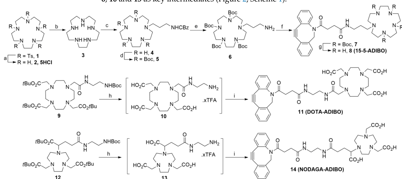
Scheme 1. Synthesis of 15-5 precursor 6 and 15-5-, DOTA- and NODAGA-ADIBO conjugates 8 , 11 and 14 : (a) (i) conc. H 2 SO 4 , 110 °C, 48 h; (ii) conc. aq. HCl, RT, 15 h; (b) aq. NaOH, toluene, Dean-Stark, overnight; (c) benzyl 3-bromopropylcarbamate ( S11 ), Et 3 N, CHCl 3 , RT, 34 h; (d) Boc 2 O, Et 3 N, CHCl 3 , RT, 18.5 h then 50 °C, 1 h; (e) H 2 , Pd/C 10%, i PrOH, RT, 48 h; (f) ADIBO-NHS S10 , DIPEA, CH 3 CN, RT, 30 h; (g) TFA, anisole, CH 2 Cl 2 , 0 °C, 2 h then RT, 1 h; (h) TFA, anisole, −10 °C then RT, 20–23 h; (i) ADIBO-NHS S10 , DIPEA, DMSO, RT, 2.5–3 h.
