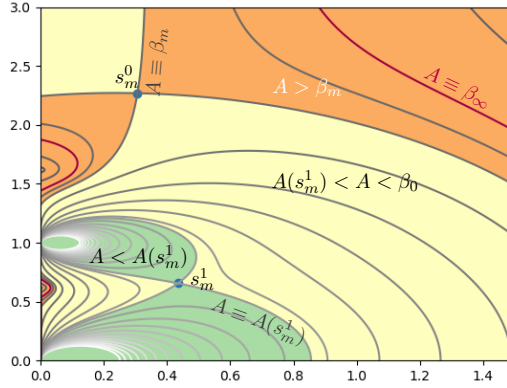
(A) Level sets, stationary points and paths of integration for the function A(\cdot, \lambda_m, t) for \lambda_m = 1
