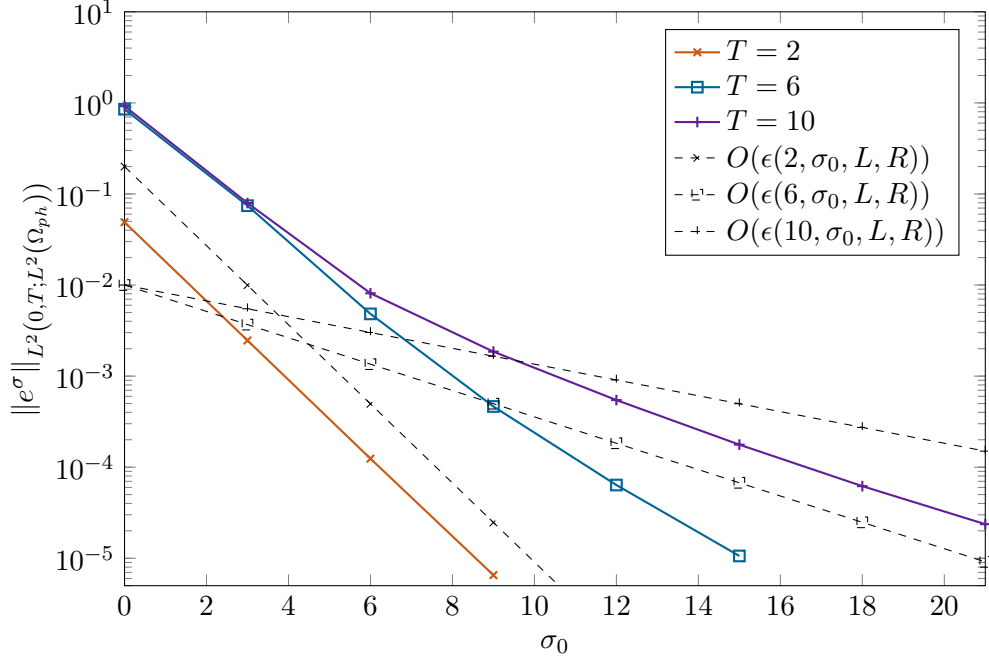
FIGURE 11. Experiment 1: Convergence of the PML-truncation for propagating waves with respect to the damping parameter. The discretization error is \approx 10^{-6} .
