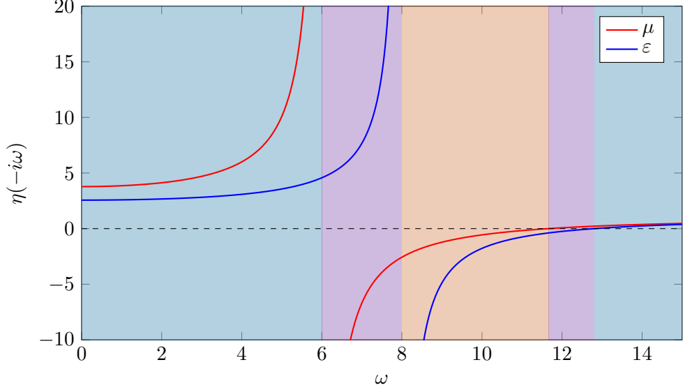
FIGURE 10. Materials used in the numerical experiments. The colors indicate the regions where we expect propagating, backward and evanescent waves.
