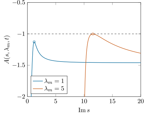
(B) A(s, \lambda_m, t) along the lines \text{Re } s = \text{Re } s_m^0 for two different values of \lambda_m .
