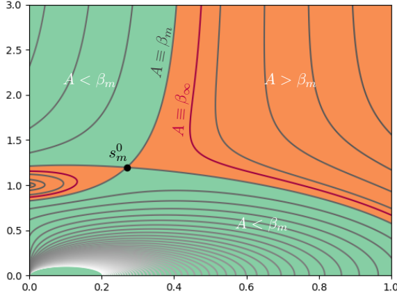
(A) level sets, stationary and paths of integration for the function A(\cdot, \lambda_m, t) for \lambda_m = 1
