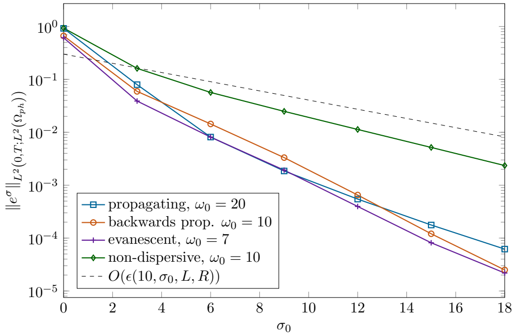
FIGURE 13. Experiment 3: Convergence of waves in different regimes. As a comparison the error of a non-dispersive waveguide is given.
