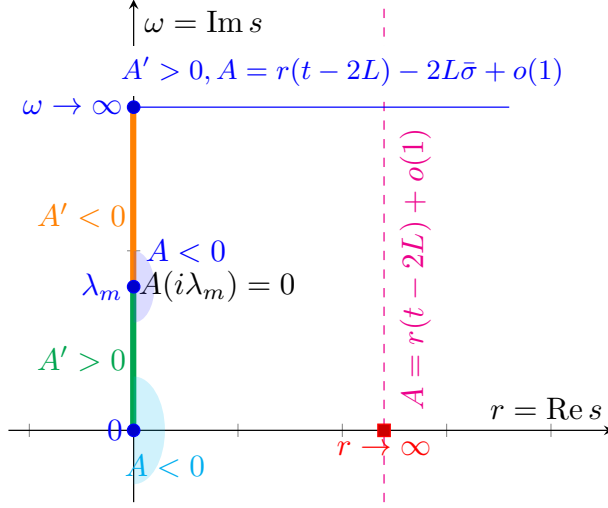
FIGURE 2. Behaviour of A in the right-half complex plane
