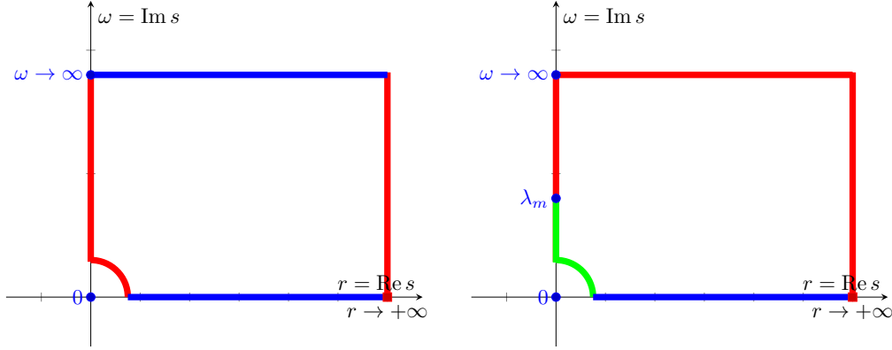
FIGURE 3. 'Forbidden' components of the boundary of the domain D_{\varepsilon, R} , for \varepsilon sufficiently small and R sufficiently large. Left: the components of boundaries of D_{\varepsilon, R} that cannot be crossed by level sets A(s, \lambda_m, t) = \text{const} > 0 are marked in red, and those that can be crossed at most once in blue. Right: the components of boundaries of D_{\varepsilon, R} that cannot be crossed by level sets A(s, \lambda_m, t) = \text{const} \leq -2L\bar{\sigma} are marked in red, and those that can be crossed at most once in blue (resp. green).
