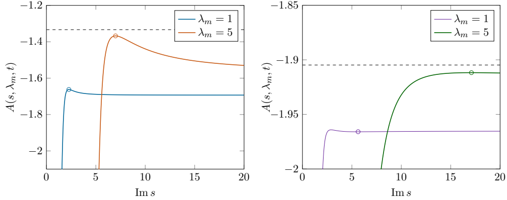
(B) A(s, \lambda_m, t) along the lines \text{Re } s = \text{Re } s_m^0 for two different values of \lambda_m and t = 3 (left) and t = 2.1 (right). The circles mark the (imaginary parts) of the saddle points and the dashed line the global bound \beta_\infty .
