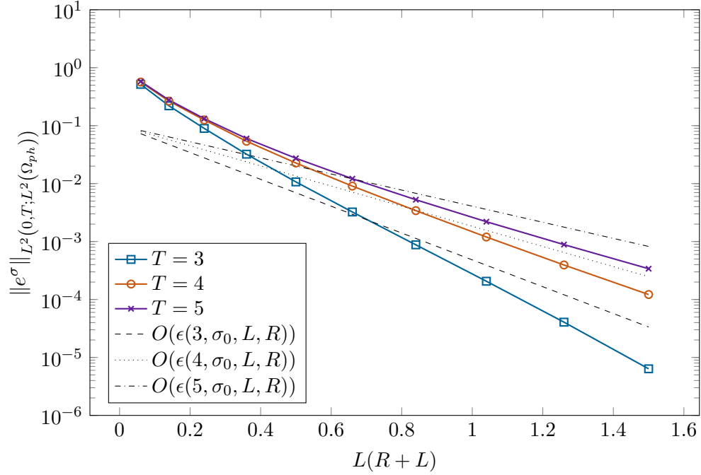
FIGURE 12. Experiment 2: Convergence of the PML-truncation for propagating waves with respect to the PML thickness. The discretization error is \approx 10^{-6} .
