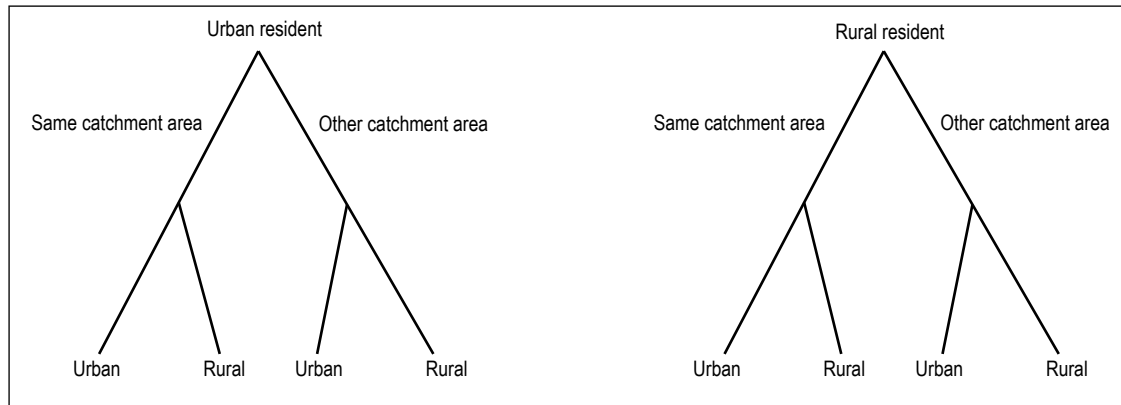
Figure I – Decision tree
