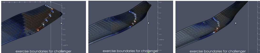
Figure 6: Exercise boundaries of the challenger. (X-axis represents the 10y swap rate; Y-axis the 10y-2y swap rate spread; the Z-axis are the range accrual's valuations).
