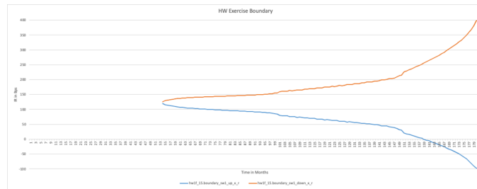
Figure 8: Exercise boundaries of the champion. (X-axis time in months to maturity; Y-axis 10y swap rate).
