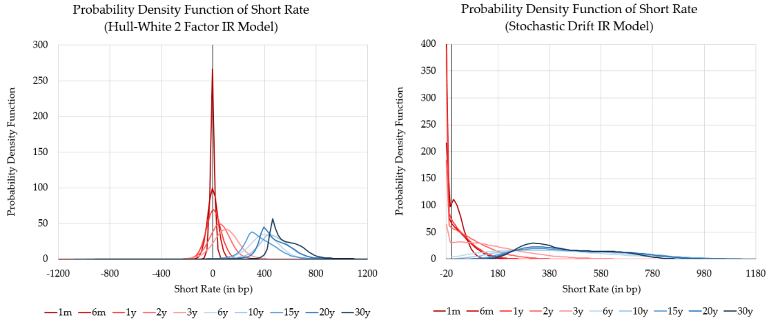
Figure 4: Probability densities of the USD short rate computed using the HW (left) and SD (right) models. Probability densities of the USD short rate computed using the champion (left) HW model and challenger (right) SD model.
