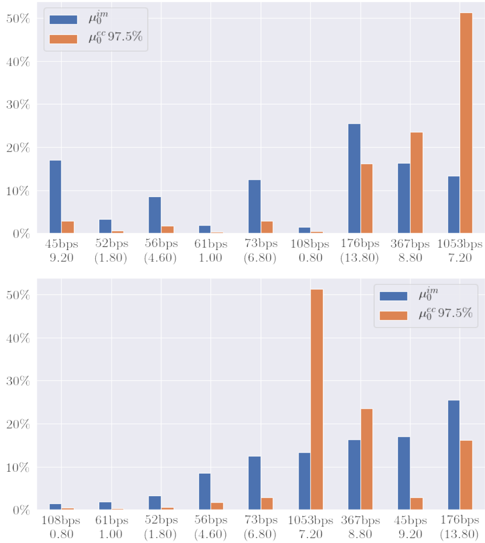
Figure 7: Time-0 default fund allocation based on member initial margin and member decremental EC^{ccp} . Bottom: Members ordered by increasing position |\nu_i| . Top: Members ordered by increasing credit spread \Sigma_i . ■
