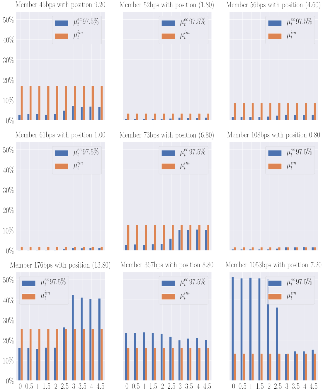
Figure 8: Default fund allocation weights term structures based on initial margins ( in orange ) versus member decremental EC^{cp} ( in blue ), for each member, ordered from left to right and top to bottom per increasing credit spread, as a function of time t = 0, \dots, 4.5 . ■
