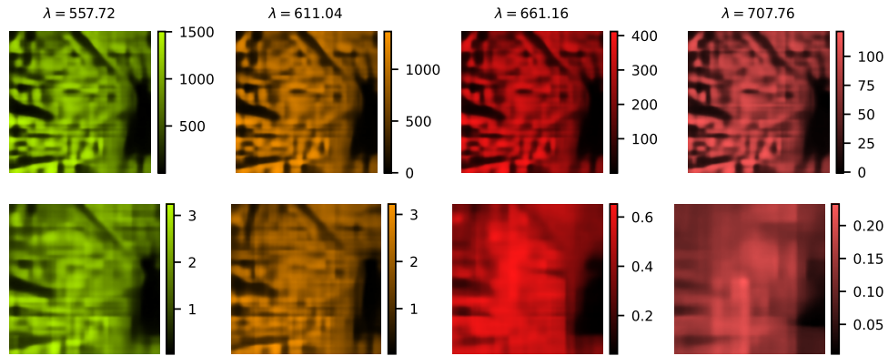
Fig. S22. Reconstruction of four spectral bins (top) and channels (bottom) using a DC-Net trained for K = 512 measurements.
