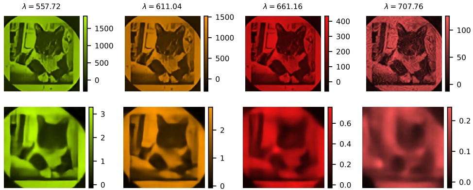
Fig. S26. Reconstruction of four spectral bins (top) and channels (bottom) using a DC-Net trained for K = 4096 measurements.
