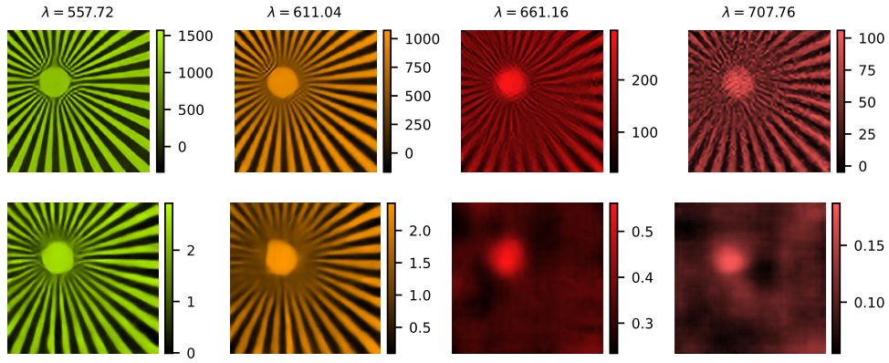
Fig. S11. Reconstruction of four spectral bins (top) and channels (bottom) using a DC-Net trained for K = 4096 measurements.
