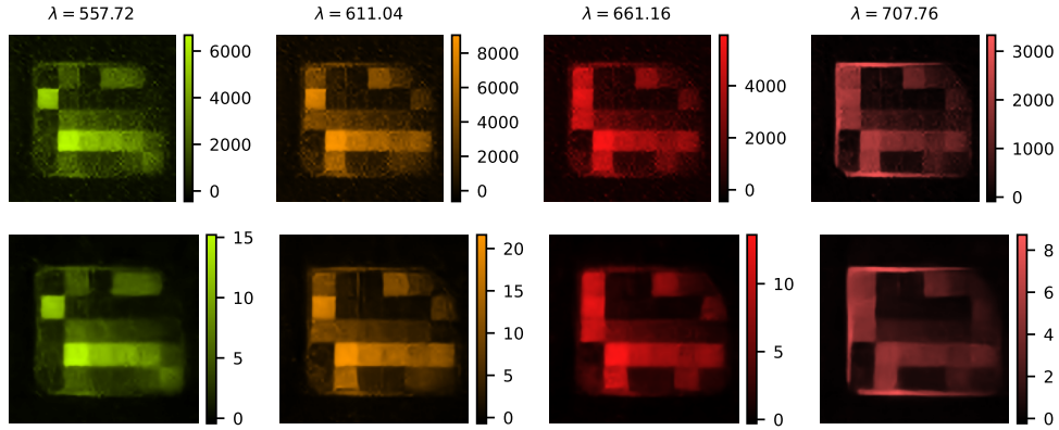
Fig. S38. Reconstruction of four spectral bins (top) and channels (bottom) using a DC-Net trained for K = 4096 measurements.
