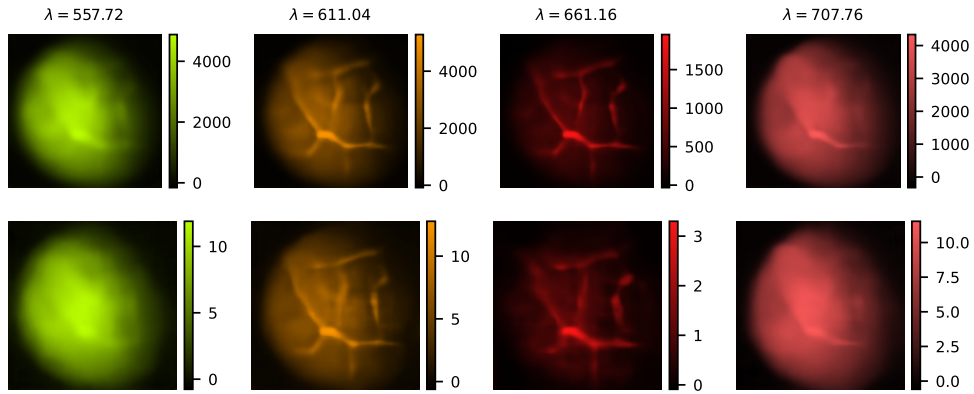
Fig. S42. Reconstruction of four spectral bins (top) and channels (bottom) using a DC-Net trained for K = 1024 measurements.
