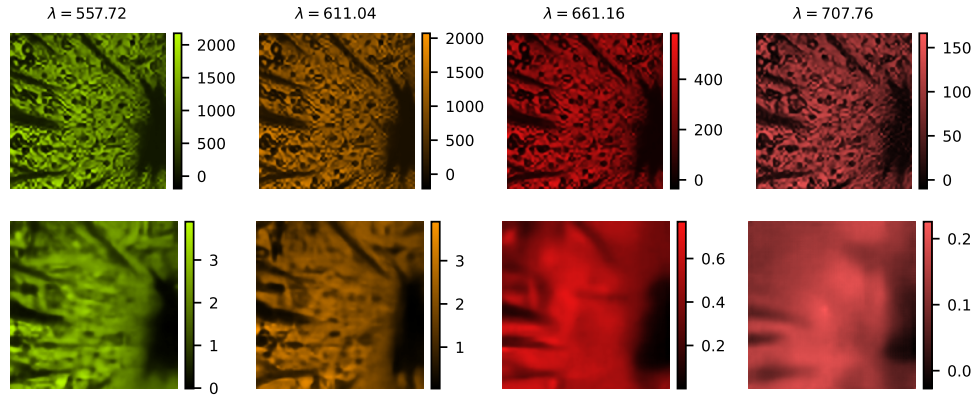
Fig. S20. Reconstruction of four spectral bins (top) and channels (bottom) using a DC-Net trained for K = 4096 measurements.
