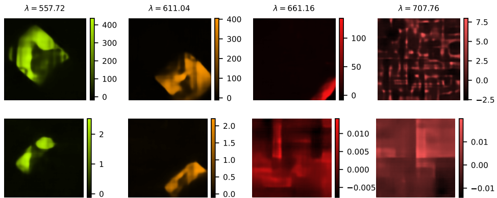
Fig. S31. Reconstruction of four spectral bins (top) and channels (bottom) using a DC-Net trained for K = 512 measurements.
