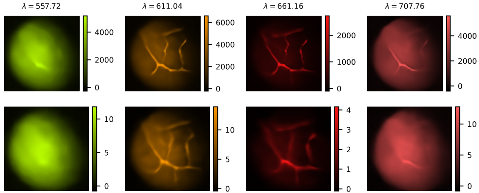
Fig. S41. Reconstruction of four spectral bins (top) and channels (bottom) using a DC-Net trained for K = 4096 measurements.
