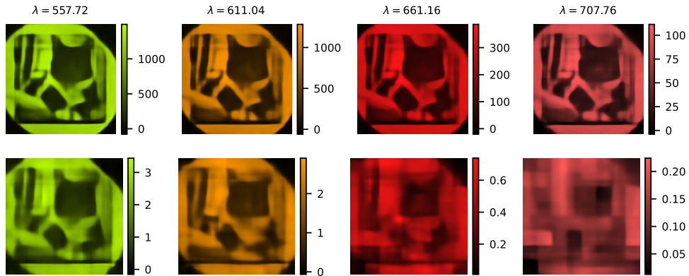
Fig. S28. Reconstruction of four spectral bins (top) and channels (bottom) using a DC-Net trained for K = 512 measurements.
