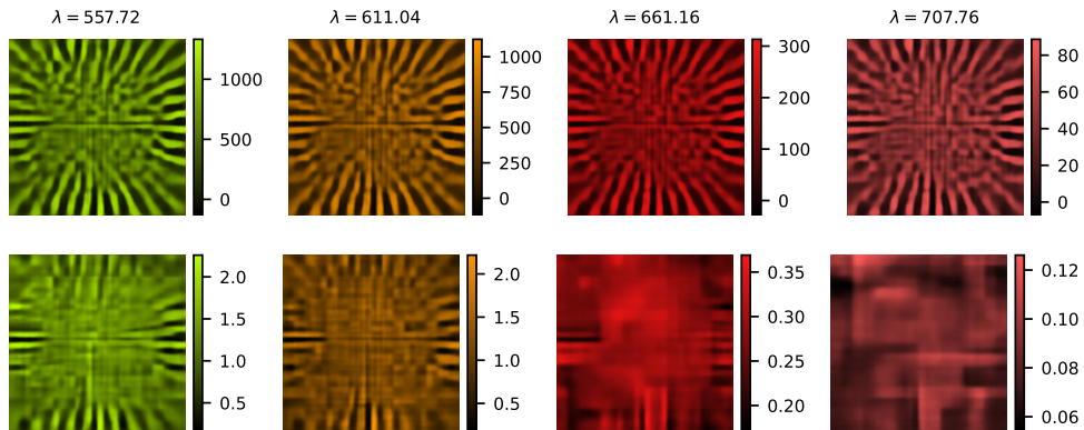
Fig. S10. Reconstruction of four spectral bins (top) and channels (bottom) using a DC-Net trained for K = 512 measurements.
