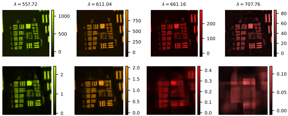
Fig. S3. Reconstruction of four spectral bins (top) and channels (bottom) using a DC-Net trained for K = 1024 measurements.
