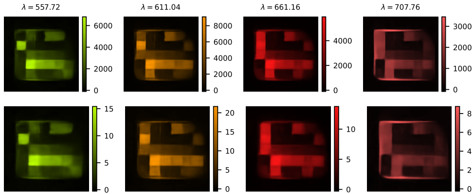
Fig. S39. Reconstruction of four spectral bins (top) and channels (bottom) using a DC-Net trained for K = 1024 measurements.
