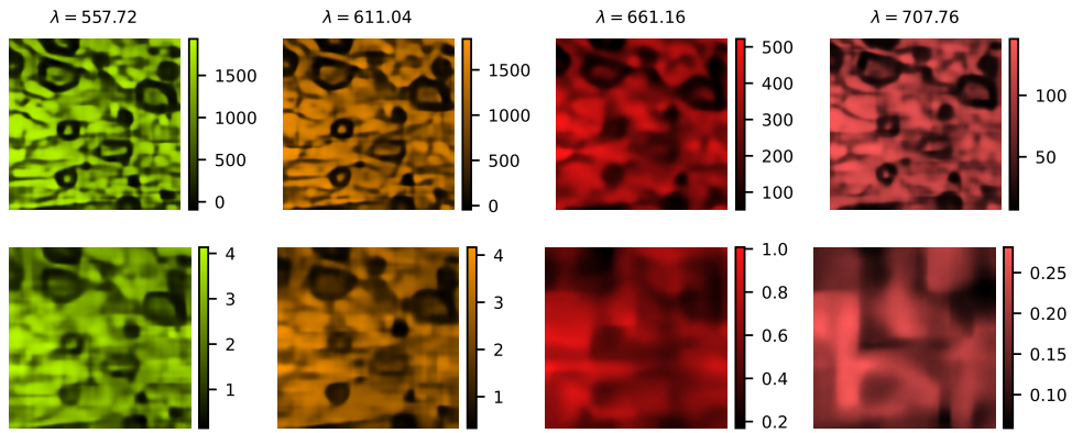
Fig. S24. Reconstruction of four spectral bins (top) and channels (bottom) using a DC-Net trained for K = 1024 measurements.
