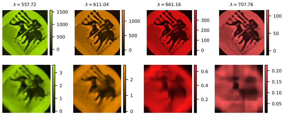
Fig. S33. Reconstruction of four spectral bins (top) and channels (bottom) using a DC-Net trained for K = 1024 measurements.
