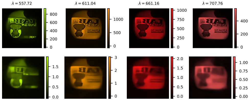
Fig. S44. Reconstruction of four spectral bins (top) and channels (bottom) using a DC-Net trained for K = 4096 measurements.
