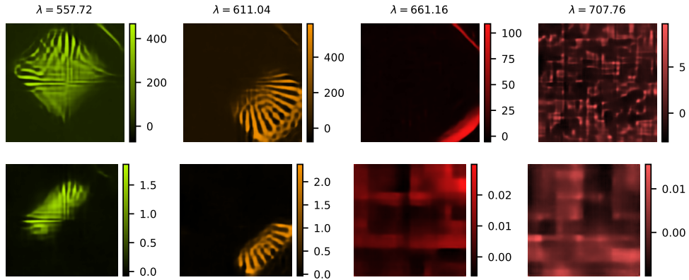
Fig. S15. Reconstruction of four spectral bins (top) and channels (bottom) using a DC-Net trained for K = 1024 measurements.
