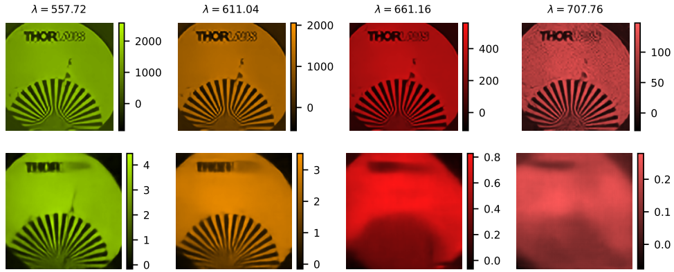
Fig. S17. Reconstruction of four spectral bins (top) and channels (bottom) using a DC-Net trained for K = 4096 measurements.
