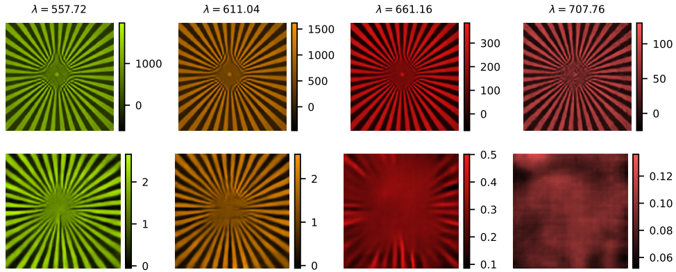
Fig. S8. Reconstruction of four spectral bins (top) and channels (bottom) using a DC-Net trained for K = 4096 measurements.
