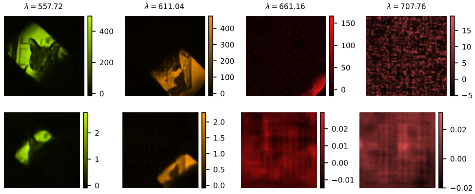
Fig. S29. Reconstruction of four spectral bins (top) and channels (bottom) using a DC-Net trained for K = 4096 measurements.
