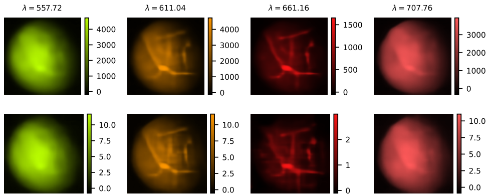
Fig. S43. Reconstruction of four spectral bins (top) and channels (bottom) using a DC-Net trained for K = 512 measurements.
