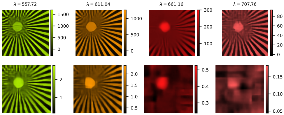
Fig. S12. Reconstruction of four spectral bins (top) and channels (bottom) using a DC-Net trained for K = 1024 measurements.
