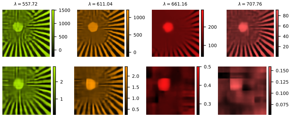
Fig. S13. Reconstruction of four spectral bins (top) and channels (bottom) using a DC-Net trained for K = 512 measurements.
