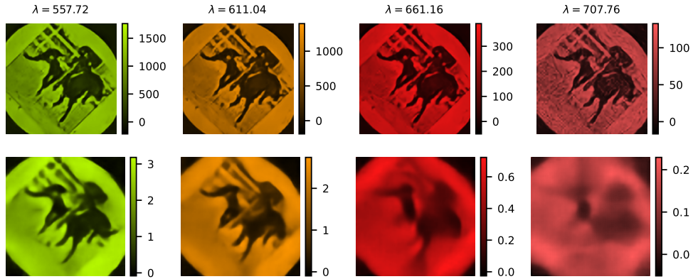
Fig. S32. Reconstruction of four spectral bins (top) and channels (bottom) using a DC-Net trained for K = 4096 measurements.
