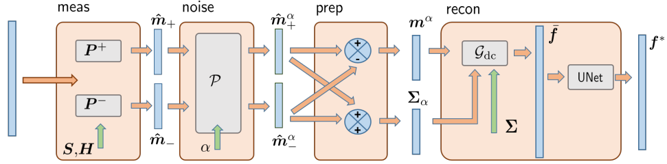
Fig. S1. Overview of the DC-Net reconstruction algorithm as implemented using four specific SPYRIT core modules. meas represents the measurement operator, noise the noise model, prep the preprocessing step, and recon the reconstruction step.
