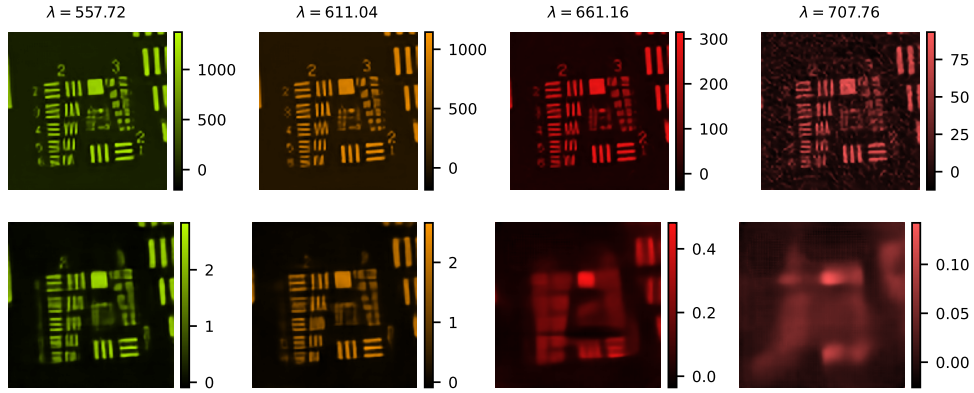
Fig. S2. Reconstruction of four spectral bins (top) and channels (bottom) using a DC-Net trained for K = 4096 measurements.
