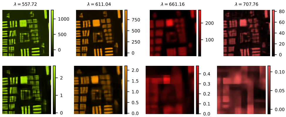
Fig. S6. Reconstruction of four spectral bins (top) and channels (bottom) using a DC-Net trained for K = 1024 measurements.
