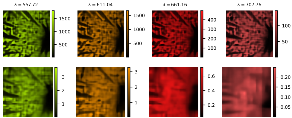
Fig. S21. Reconstruction of four spectral bins (top) and channels (bottom) using a DC-Net trained for K = 1024 measurements.
