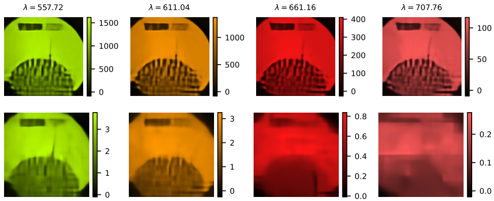
Fig. S19. Reconstruction of four spectral bins (top) and channels (bottom) using a DC-Net trained for K = 512 measurements.
