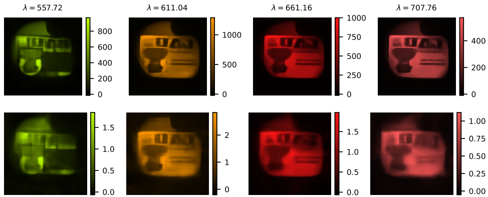
Fig. S45. Reconstruction of four spectral bins (top) and channels (bottom) using a DC-Net trained for K = 1024 measurements.
