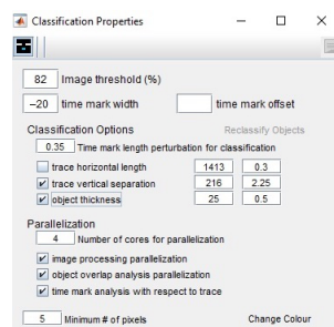
Figure 9. Threshold parameters for seismogram classification in DigitSeis.
