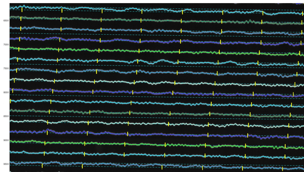
Figure 12. Results of the paper-based seismogram vectorisation processed by DigitSeis. (a) Digitised traces upon completion of the automated vectorisation. Some time gaps in the upper left part of the image were too small and not clearly visible for the automatic discrimination between the trace and the dark background. In these cases, gaps required manual correction to identify time intervals. (b) The enlarged view of the automatically recognised digitised traces displayed by the lines of various colours, zero-lines for each trace (cyan, dashed lines, numbered from top to bottom) and time gaps (vertical yellow dashes).
