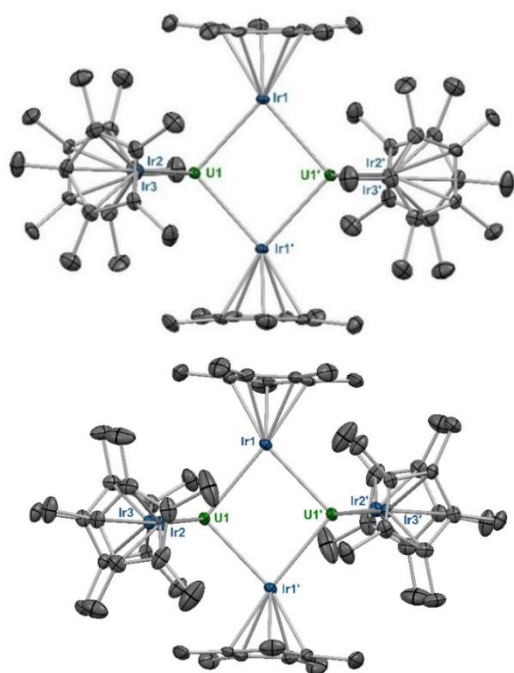
Figure 2. Solid-state molecular structures of 3s and 3e . Ellipsoids are presented at the 50% probability level. Hydrogen atoms have been omitted for clarity. Selected bond distances (Å) and angles (deg) for 3s : U1–Ir1 2.8135(3), U1–Ir2 2.9718(3), U1–Ir3 2.9653(3), U1–U1' 3.7945(4), Ir1–U1–Ir2 109.34(1), Ir1–U1–Ir1' 95.70(1), Ir2–U1–Ir3 113.47(1), U1–Ir2–Cp* centroid 175.55(1), Ir1'–Ir1–Cp* centroid 179.06(1). Selected bond distances (Å) and angles (deg) for 3e : U1–Ir1 2.8392(3), U1–Ir2 2.9899(3), U1–Ir3 2.9728(3), U1–U1' 3.7819(4), Ir1–U1–Ir2 113.64(1), Ir1–U1–Ir1' 96.25(1), Ir2–U1–Ir3 120.85(1), U1–Ir2–Cp* centroid 177.89(1), Ir1'–Ir1–Cp* centroid 174.19(1).
