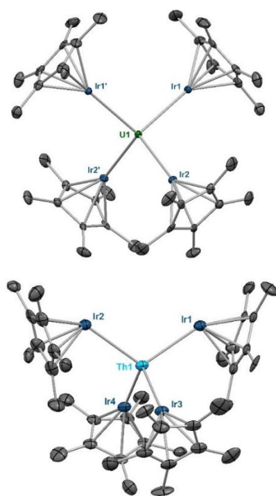
Figure 1. Solid-state molecular structures of 1 (top) and 2 (bottom). Ellipsoids are presented at the 50% probability level. Hydrogen atoms and co-crystallized solvent molecules have been omitted for clarity. Selected bond distances (Å) and angles (deg) for 1 : U1–Ir1 2.9508(5), U1–Ir2 2.9587(5), Ir1–U1–Ir2 106.40(1), Ir1–U1–Ir2 104.24(2), Ir1–U1–Ir2' 118.94(1), U1–Ir1–Cp* centroid 173.61(1). Selected bond distances (Å) and angles (deg) for 2 : Th1–Ir1 2.9639(11), Th1–Ir2 2.9827(10), Th1–Ir3 3.0153(12), Th1–Ir4
