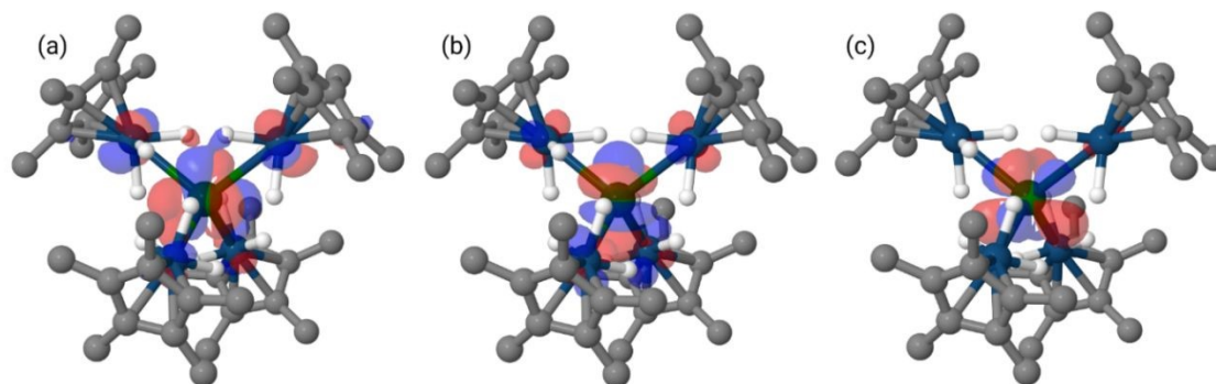
Figure 4. Renderings of the calculated SOMOs (a, b) and LUMO (c) of 1 (isovalue = 0.03)
