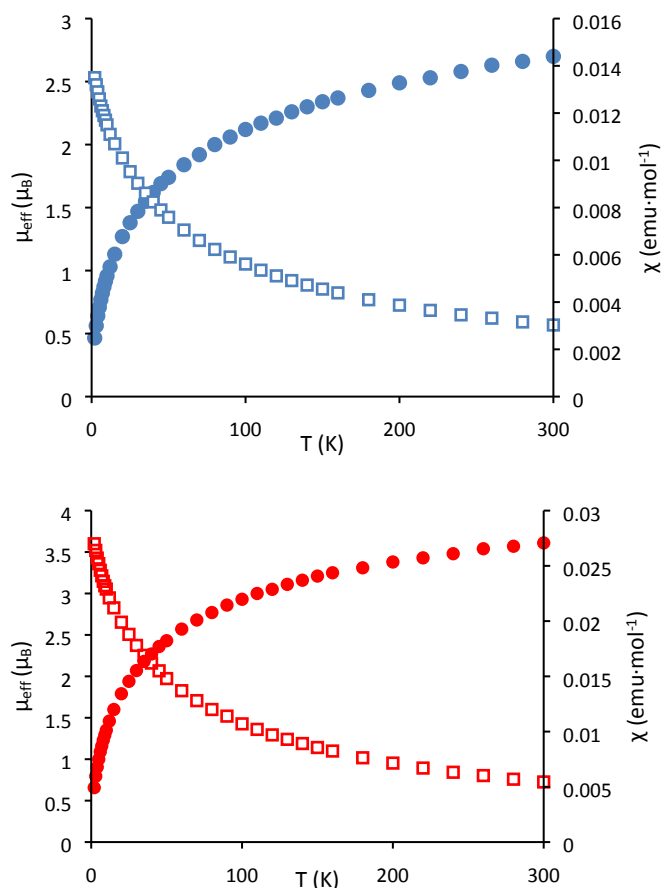
Figure 3. Temperature-dependent SQUID magnetization data (4 T) for 1 (blue) and 3 (red) plotted as \mu_{\text{eff}} (filled circles) and \chi (open squares) versus temperature. Data were corrected for diamagnetic contributions.
