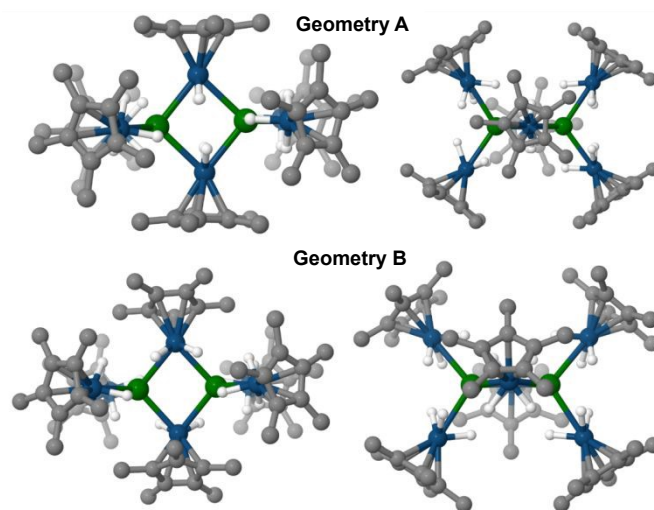
Figure 5. Calculated geometries for two local energy minima of 3 . The hydrides on the bridging [IrCp^*H_2]^{2-} fragments for Geometry A (top) are equidistant from the U atoms, and extend outward from the Ir atom so that the H–Ir–H and Ir–U–Ir planes are nearly perpendicular. In Geometry B (bottom), the hydrides on the [IrCp^*H_2]^{2-} fragments bridge the Ir–U interactions on the same side of the U–Ir–U plane, resulting in significant tilting of the Cp* planes with respect of the U_2Ir_2 plane.
