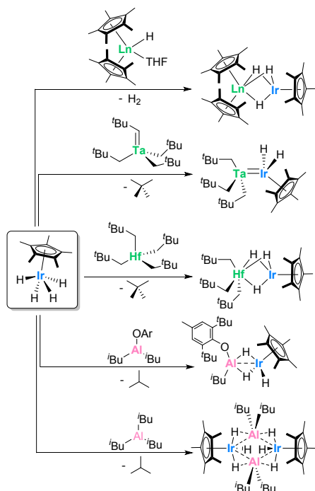
Scheme 1. Previously reported syntheses of reactive multimetallic complexes from \text{IrCp}^*\text{H}_4 . 40,43,49,50,51
