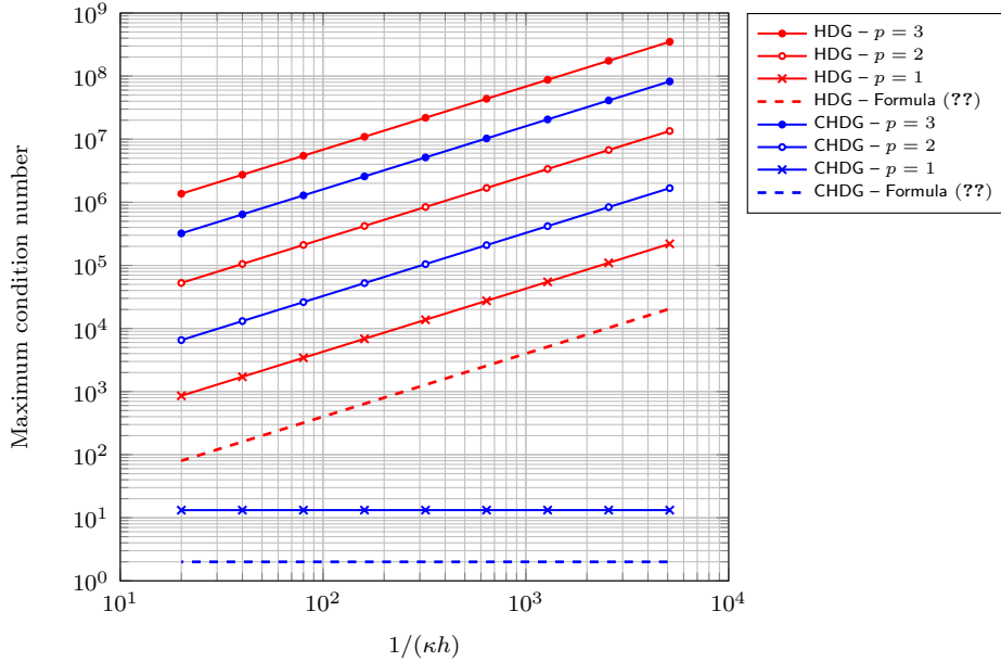
Figure 2: Maximum condition number of the local matrices with HDG (red curves) and CHDG (blue curves) as a function of 1/(\kappa h) for basis functions with polynomial degrees p = 1, 2 and 3 .
