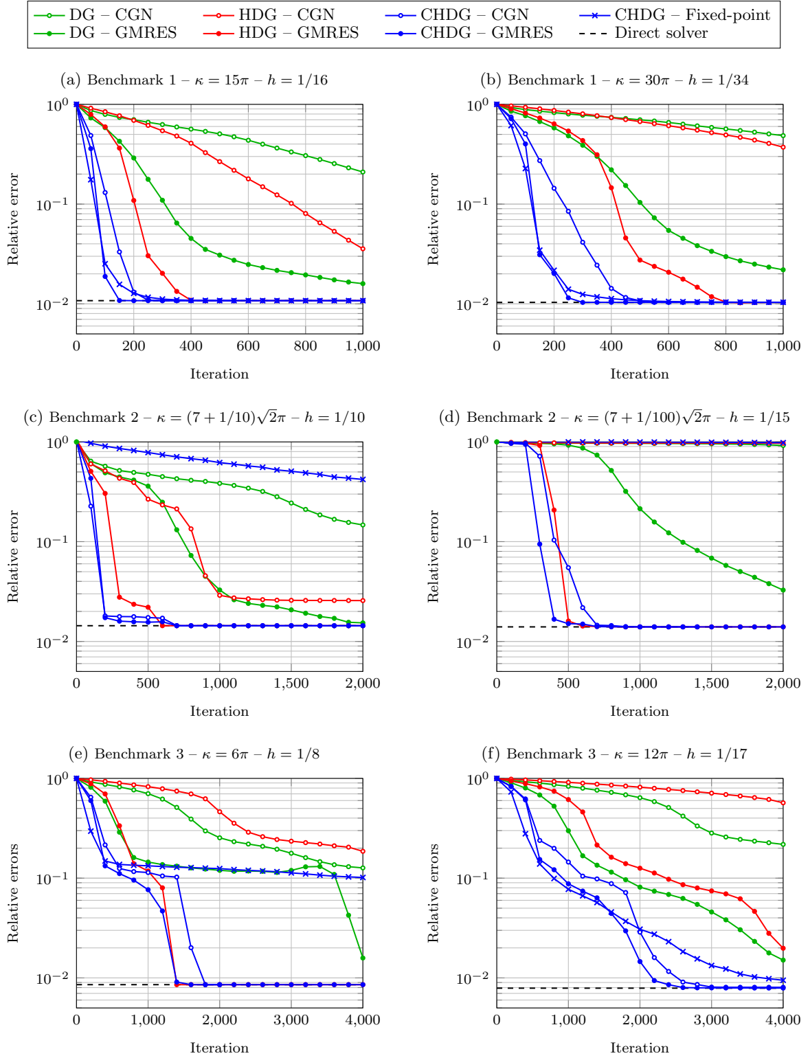
Figure 4: Error history for the three benchmarks with different iterative schemes and different DG schemes. The dashed horizontal lines correspond to the relative errors obtained with a direct solver.
