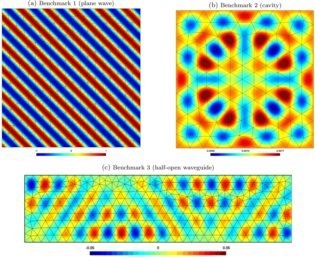
Figure 1: Snapshots of the real part of the solution for the three benchmarks with the default parameters.
