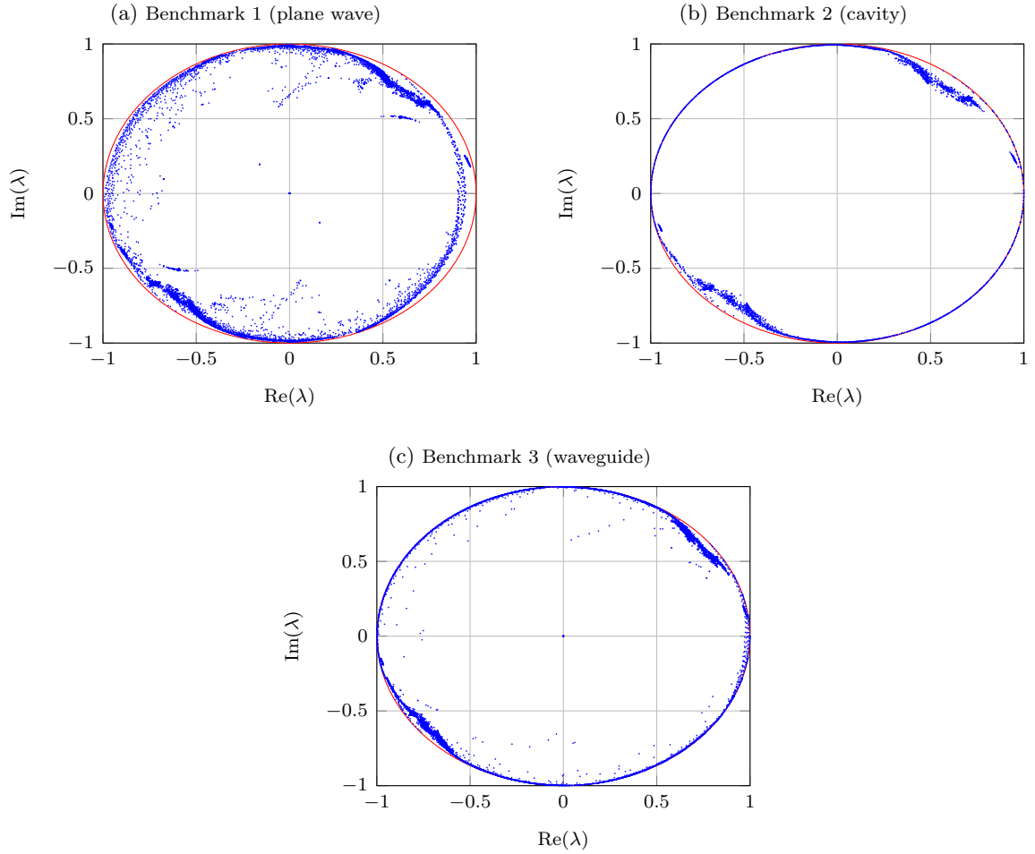
Figure 3: Spectrum of the iteration matrix \mathbf{\Pi S} of the fixed-point iterative scheme for the three benchmarks with the default parameters and the CHDG method. The unit circle is plotted in red.
