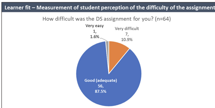
Figure 1. Learner fit
