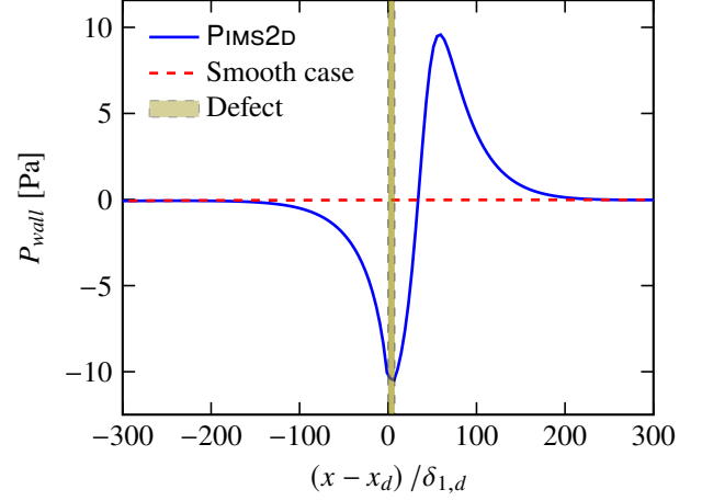
Figure 3: Pressure distribution at the wall in the boundary layer.
