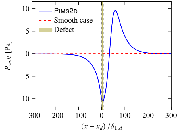
Figure 3: Pressure distribution at the wall in the boundary layer.
