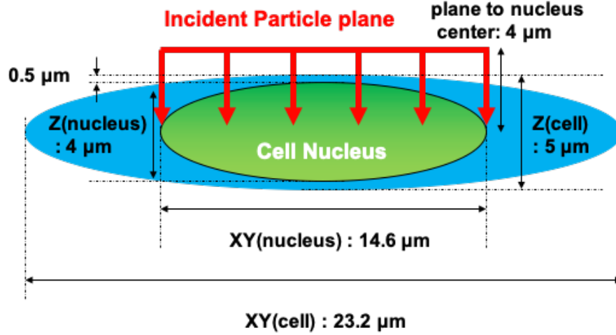
FIG. 1. Geometrical model of a cell nucleus imitating a Chinese hamster V79 cell in the simulations.
