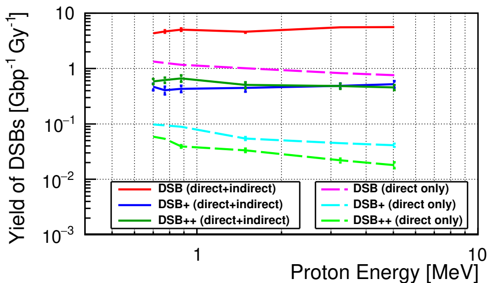
FIG. 2. The average yield of DSBs for each damage type, as categorized by Nikjoo’s definition 7 . The results with the full simulation were labeled as “direct+indirect”, and the results of the simulations without the chemistry interface were labeled as “direct only”.
