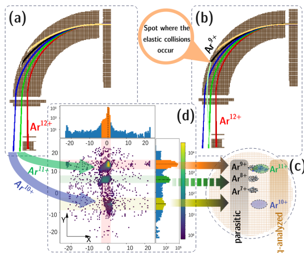
Figure 3. A comparison of SIMION simulations (a–c) and experiment (d) for the case of \text{Ar}^{12+} recorded by the Faraday Cup (a) with the trajectories of \text{Ar}^{11+} and \text{Ar}^{10+} ions alone; (b) with the trajectory of the \text{Ar}^{9+} beam suffering an elastic collision; (c) peaks expected on the 2D detector.
