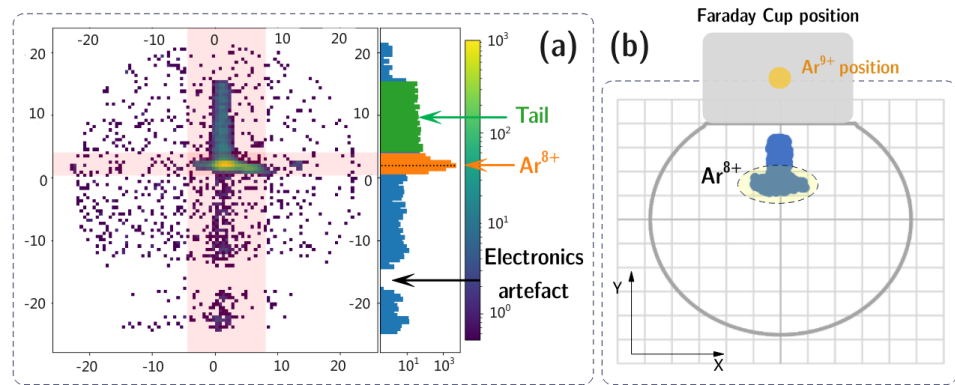
Figure 2. A recorded MCP image with the use of \text{Ar}^{9+} as the primary beam exhibits the \text{Ar}^{8+} peak and its tail (a). Results of SIMION simulations carried out with the same voltages and beam parameters (b). The horizontal line where no detection occur has been found to be an electronic artefact of the MCP.
