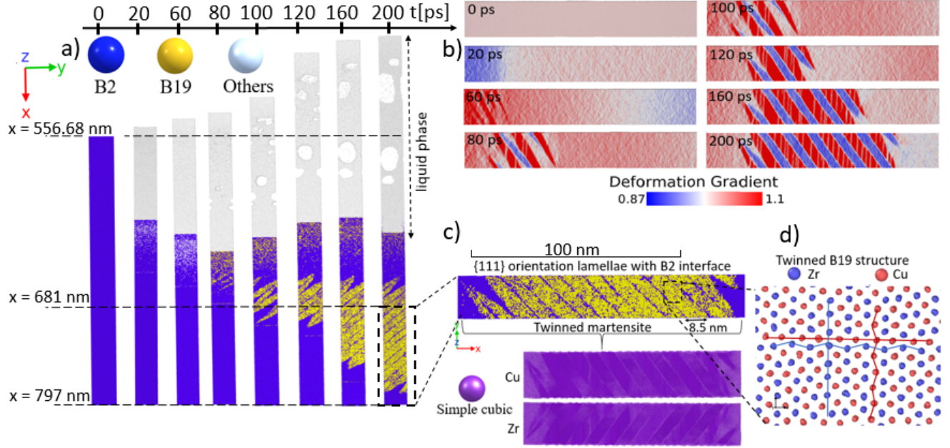
Figure 2. Snapshots of the atomic configurations evolution in figure a) at several times : 0 ps, 20 ps, 60 ps, 80 ps, 100 ps, 120 ps, 160 ps, and 200 ps in B_2 - Cu_{50}Zr_{50} target during ultrafast laser irradiation of \tau = 100 fs pulse duration and F_{abs} = 160 mJ/cm 2 absorbed fluence. The atoms are colored according to their local atomic structure of the binary alloy by using the PTM, the double dashed arrow in the upper part of target shows the liquefied surface. b) Deformation gradient in the transformed zone following the x direction at different times computed by the method described in [77]. c) Zoom on the dashed region where the PTM algorithm is applied on each sub-lattice monoatomic lattice showing twinned martensite transformation. d) Enlarged view of the chemical species of the new twinned-B19 phase emergence after the irradiation.
