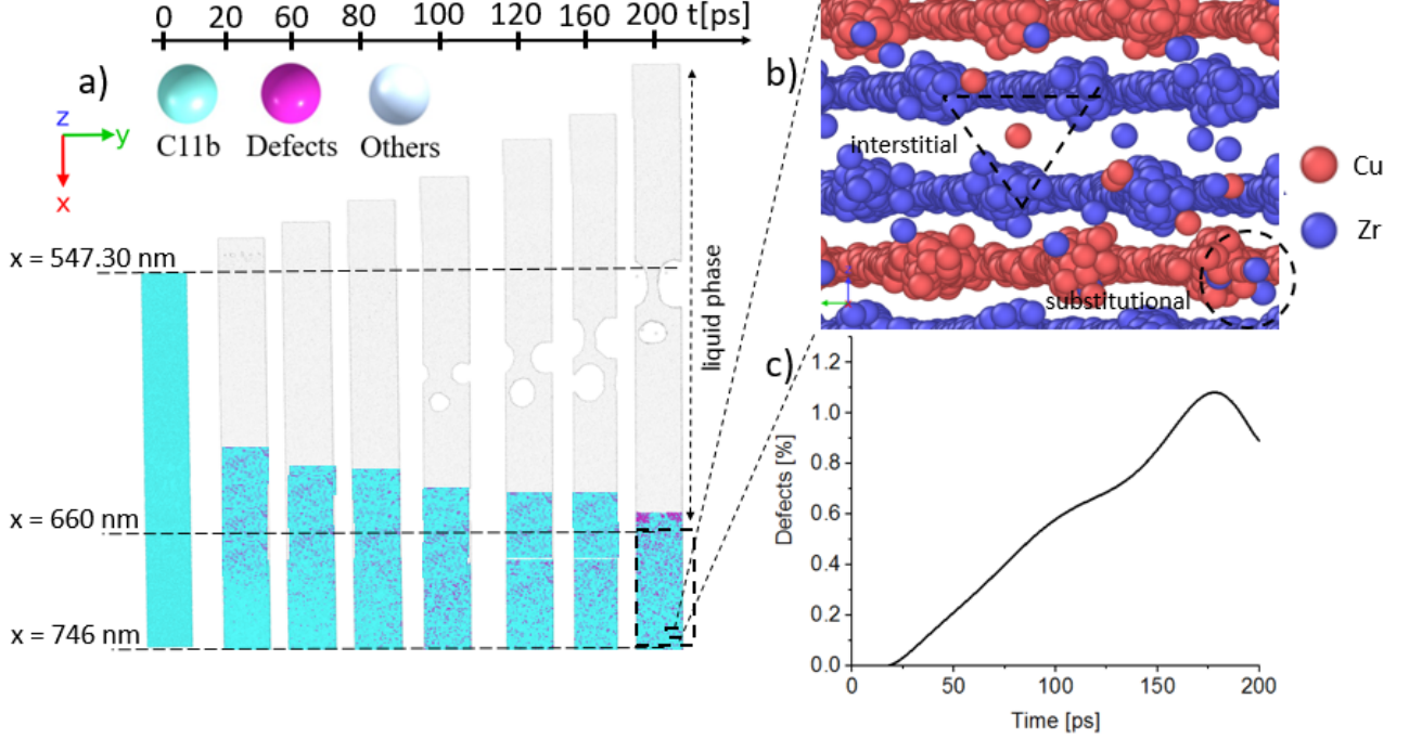
Figure 5. Snapshots of atomic configurations evolution in figure a) at several times: 0 ps, 20 ps, 60 ps, 80 ps, 100 ps, 120 ps, 160 ps, and 200 ps in the C11_b - Cu_{33.3}Zr_{66.7} sample target during ultrafast laser irradiation of \tau = 100 fs pulse duration and F_{abs} = 160 mJ/cm 2 of absorbed fluence, the double dashed arrow in the upper part of target shows the liquefied surface. The atoms are colored according to their local atomic structure using PTM algorithm. b) Enlarged view of interstitial and substitutional defects formation in subsurface within C11_b - Cu_{33.3}Zr_{66.7} target after the irradiation at different times. c) Temporal defects ratio evolution in Cu_{33.3}Zr_{66.7} ( C11_b ) target sorted according to the displacement vector \delta y > 1 Å. Atoms satisfying this condition are expected to be in defective positions, this is achieved using displacement vectors analysis [83].
