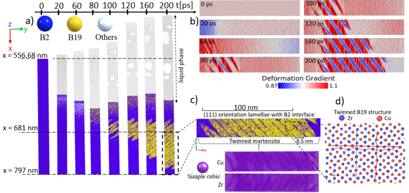
Figure 2. Snapshots of the atomic configurations evolution in figure a) at several times : 0 ps, 20 ps, 60 ps, 80 ps, 100 ps, 120 ps, 160 ps, and 200 ps in B 2 -Cu 50 Zr 50 target during ultrafast laser irradiation of \tau = 100 fs pulse duration and F_{\text{abs}} = 160 mJ/cm 2 absorbed fluence. The atoms are colored according to their local atomic structure of the binary alloy by using the PTM, the double dashed arrow in the upper part of target shows the liquefied surface. b) Deformation gradient in the transformed zone following the x direction at different times computed by the method described in [77]. c) Zoom on the dashed region where the PTM algorithm is applied on each sub-lattice monoatomic lattice showing twinned martensite transformation. d) Enlarged view of the chemical species of the new twinned-B19 phase emergence after the irradiation.
