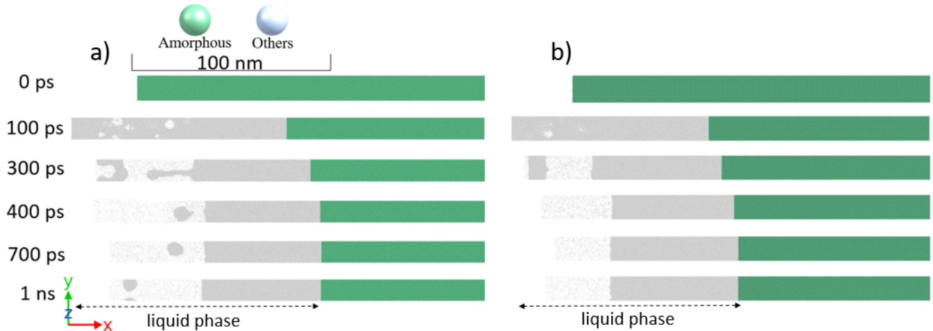
Figure 4. Snapshots of the structural evolution in the amorphous structures: a) \alpha -Cu 50 Zr 50 , and b) \alpha -Cu 33.3 Zr 66.7 using TTM-MD method at various time steps: 0 ps, 100 ps, 300 ps, 400 ps, 700 ps, and 1 ns. The atoms are colored according to their local atomic structure using PTM algorithm, two atomic contrasts are shown, the zone delimited by a double dashed arrow in the upper part of targets correspond to liquid phase and the inner part is the amorphous phase. The irradiation conditions are \tau = 100 fs pulse duration and F_{\text{abs}} = 160 mJ/cm 2 of absorbed fluence.
