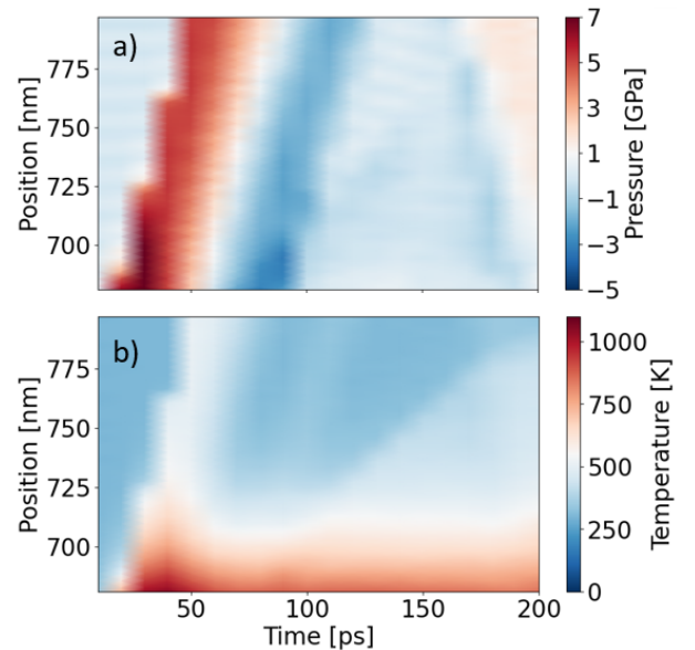
Figure 3. Spatiotemporal evolution of thermodynamic quantities in the B 2 -Cu 50 Zr 50 transformed region located in sub-surface (zoom region) area target: a) pressure, and b) lattice temperature. The initial surface position is given by x_{\text{surface}} = 556.68 nm following the x axis direction.
