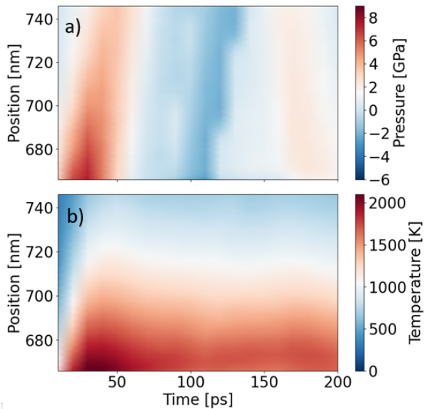
Figure 6. Spatiotemporal evolution of thermodynamic quantities in the subsurface transformed region (zoom region) : a) pressure, and b) lattice temperature evolution in (C11 b -Cu 33.3 Zr 66.7 sample target. The initial surface position is given by x_{\text{surface}} = 547.30 nm following the x axis direction.
