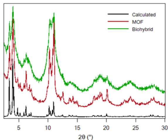
Figure 1. Powder X-Ray diffractions patterns (CuK \alpha radiation, \lambda = 1.5418 Å) of MIL-100(Fe) calculated (black), synthesized without bacterium (red) and with bacteria (green).
