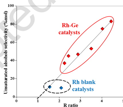
Figure 19. Unsaturated alcohols selectivity as a function of R ( R = \frac{\sum A(\text{COads on Rh}_{\geq 1+} \text{ species})}{\sum A(\text{COads on total exposed Rh species})} ) for 1wt.%Rh-xwt.%Ge/TiO 2 ( x \geq 0 ) catalysts prepared from various metal salt precursors and reduced at 300 °C.
