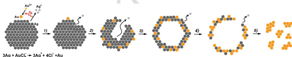
Figure 2. Schema of the morphological and structural changes at different stages of the GR reaction between a Ag particle and a HAuCl 4 aqueous solution. Adapted with permission from Ref. [18]. Copyright © 2013 John Wiley and Sons.
