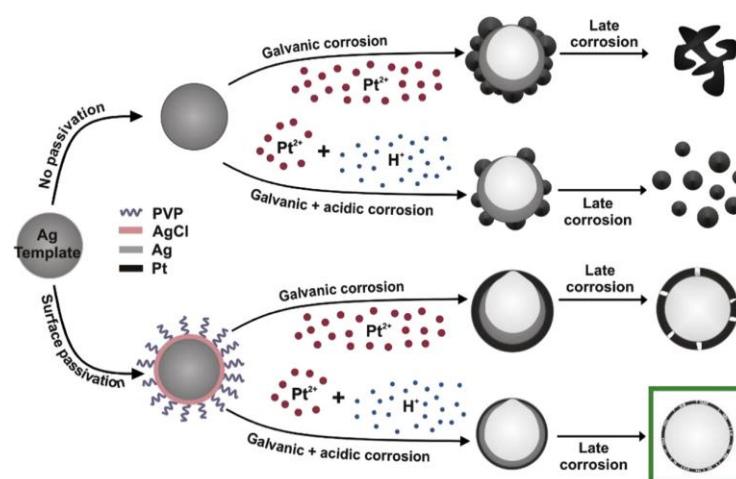
Figure 7. Schematic representation of distinct types of AgPt hollow nanoparticles obtained by galvanic replacement performed in various conditions (PVP: polyvinylpyrrolidone). Adapted with permission from Ref. [48]. Copyright © 2020 Elsevier.
