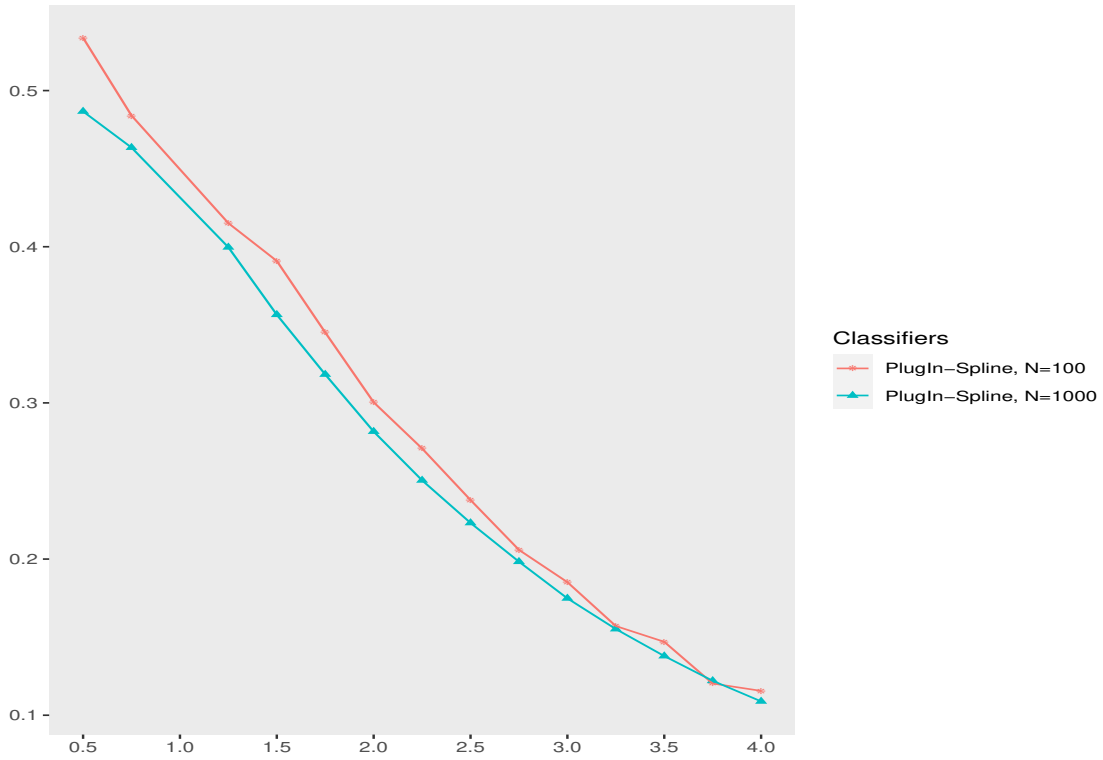
Figure 2: Risks of the plug-in classifier w.r.t values of the minimum gap \theta between the drift functions
