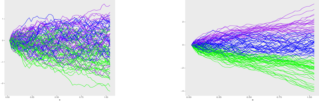
Figure 1: Dispersion of diffusion paths from model given in Table 1. Left: \theta = 1/2 , right: \theta = 4 (blue lines K = 1 , purple lines K = 2 , green lines K = 3 ); with N = 100 and n = 100 .
