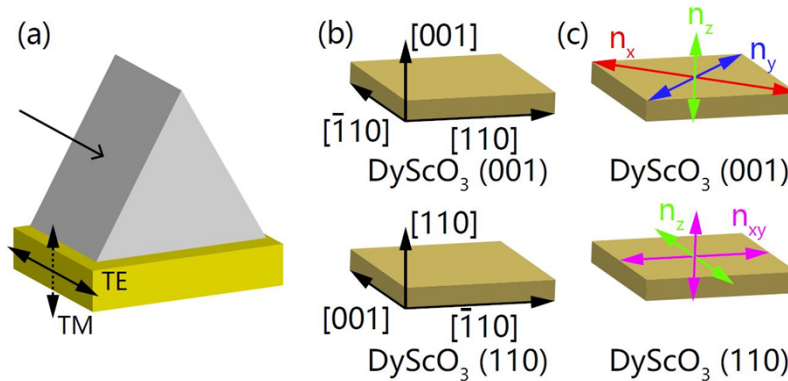
Fig. 1. (a) Schematic drawing of the prism coupling measurement setup. (b) Crystal structure and (c) refractive indices of \text{DyScO}_3 (001) and \text{DyScO}_3 (110). The crystal orientations are labeled in black, and the refractive indices are labeled in colors which correspond to the polarization directions in the prism coupling measurements.
