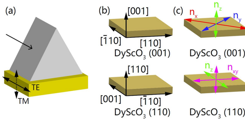
Fig. 1. (a) Schematic drawing of the prism coupling measurement setup. (b) Crystal structure and (c) refractive indices of DyScO 3 (001) and DyScO 3 (110). The crystal orientations are labeled in black, and the refractive indices are labeled in colors which correspond to the polarization directions in the prism coupling measurements.
