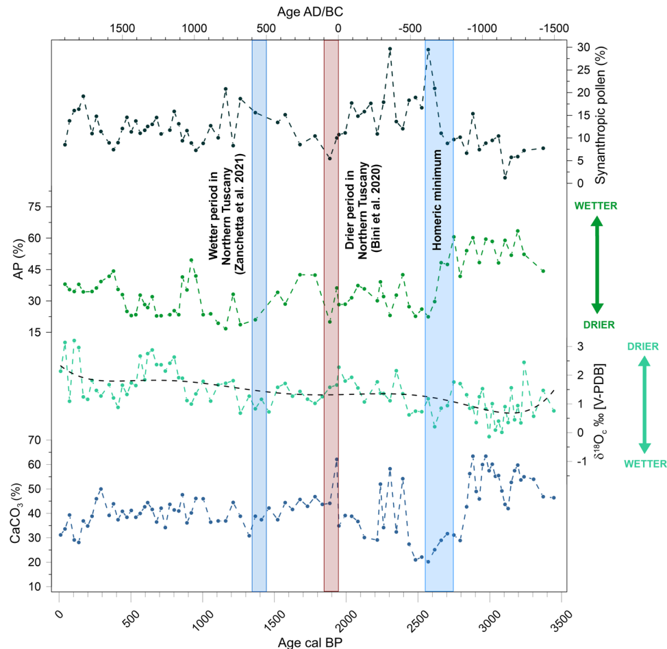
Figure 9. Synanthropic pollen percentage (calculated after Sadori et al. , 2013) compared with arboreal pollen percentage (AP) (Sadori et al. , 2013), \delta^{18}\text{O}_c (this work), and \text{CaCO}_3\% (this work) for the PG2 core for the last 3500 years. The dotted line for \delta^{18}\text{O}_c is a fit of the 6th polynomial order. Highlighted in colored squares are particular chronological intervals discussed in the text. [Color figure can be viewed at wileyonlinelibrary.com ]
