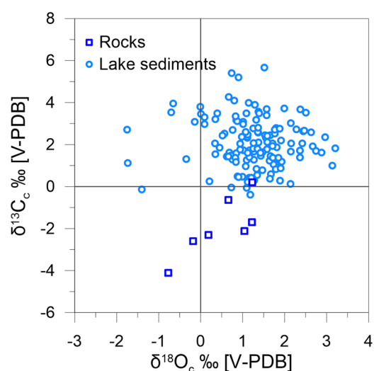
Figure 7. \delta^{13}\text{C}_\text{c} vs. \delta^{18}\text{O}_\text{c} of lacustrine carbonates and catchment rocks. Catchment rocks and lacustrine carbonates generally have no overlapping values. [Color figure can be viewed at wileyonlinelibrary.com ]
