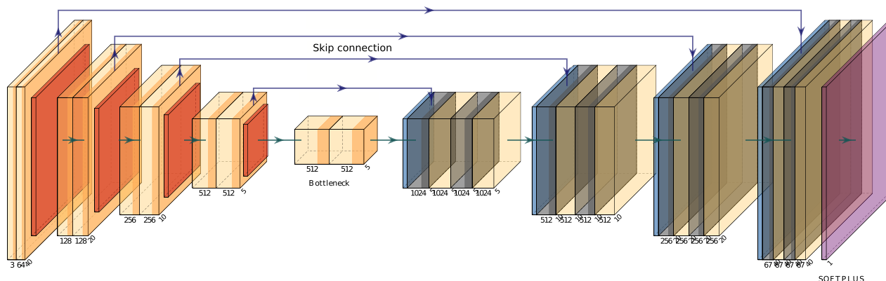
FIGURE 8. U-net architecture.
