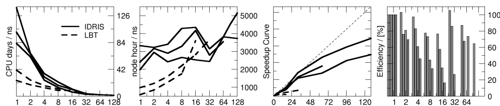
Figure 5. Benchmarks carried out at the IDRIS supercomputer center and locally at the LBT laboratory. From left to right: CPU days per nanosecond (ns), node hours per ns, speedup curve and computational efficiency.
