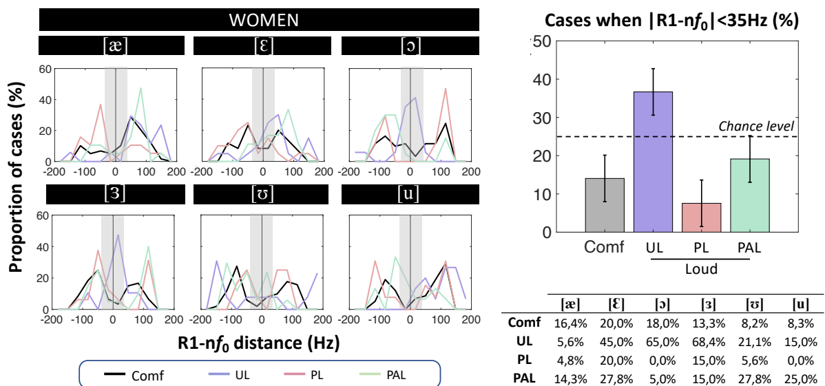
Figure 4. On the left: The distribution of frequency differences observed between the frequency of the first vocal tract resonance (R1) and the closest voice harmonic ( nf_0 ), for women pronouncing each vowel and mode of phonation (Comfortable voice and loud phonations (UL, PL, PAL)). On the right: Percentage of cases for which R1 frequencies are closer than 35 Hz to a voice harmonic, on average, and for each vowel produced by women at comfortable and loud levels. The dashed line represents the level of chance for observing such a resonance-harmonic proximity.
