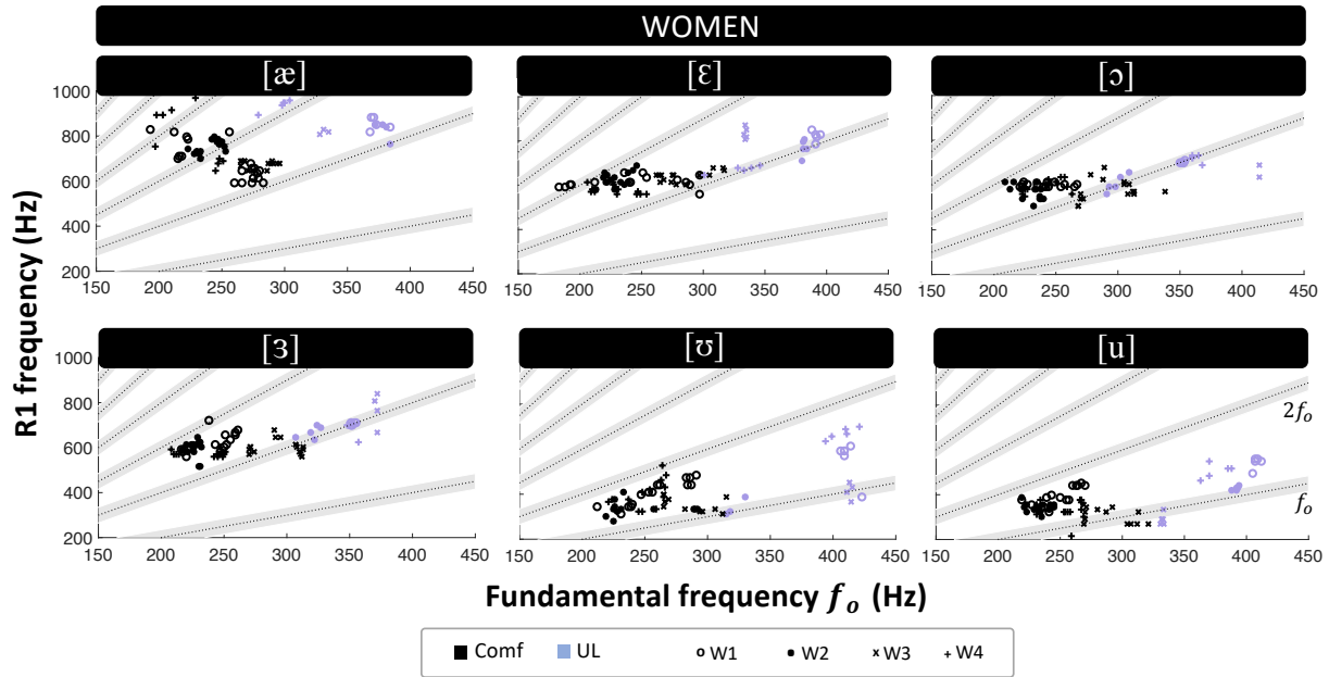
Figure 5. The relationship between values of (f_0, R1) measured simultaneously for the six vowels produced by the four women of this study (W1, W2, W3, W4), in comfortable voice (black) and ‘natural’ loud voice UL (light blue). The dashed lines represent the voice harmonics nf_0 . Shaded grey areas indicate a 70 Hz interval centered around these voice harmonics, corresponding to the typical bandwidth of vocal tract resonances (Hanna et al., 2016).
