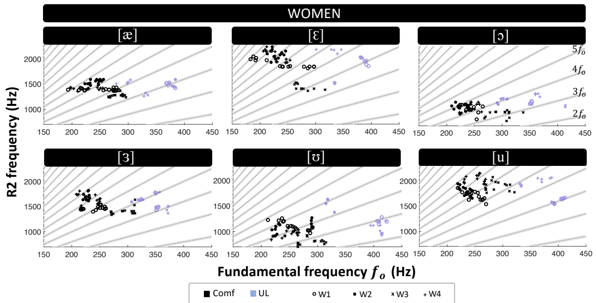
Figure 9. The relationship between values of (f_0, R2) measured simultaneously for the six vowels produced by the four women of this study (W1, W2, W3, W4), in comfortable voice (black) and ‘natural’ loud voice UL (light blue). The dashed lines represent the voice harmonics nf_0 . Shaded grey areas indicate a 70 Hz interval around these voice harmonics, corresponding to the typical bandwidth of vocal tract resonances (Hanna et al., 2016).
