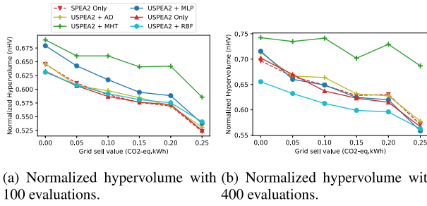
FIGURE 13. Impact of the grid sell utility parameter ( ghg_{sell} ) for the different approximation methods used with USPEA2.
